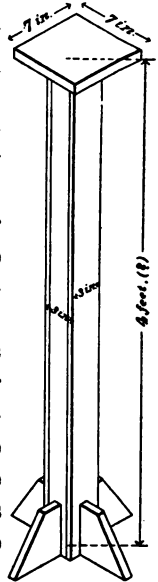
Fig. 1.—Support.
