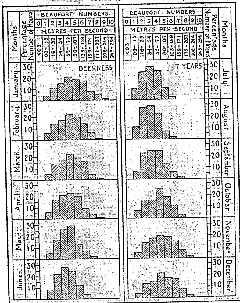
Monthly Average Wind Frequency at Deerness.
