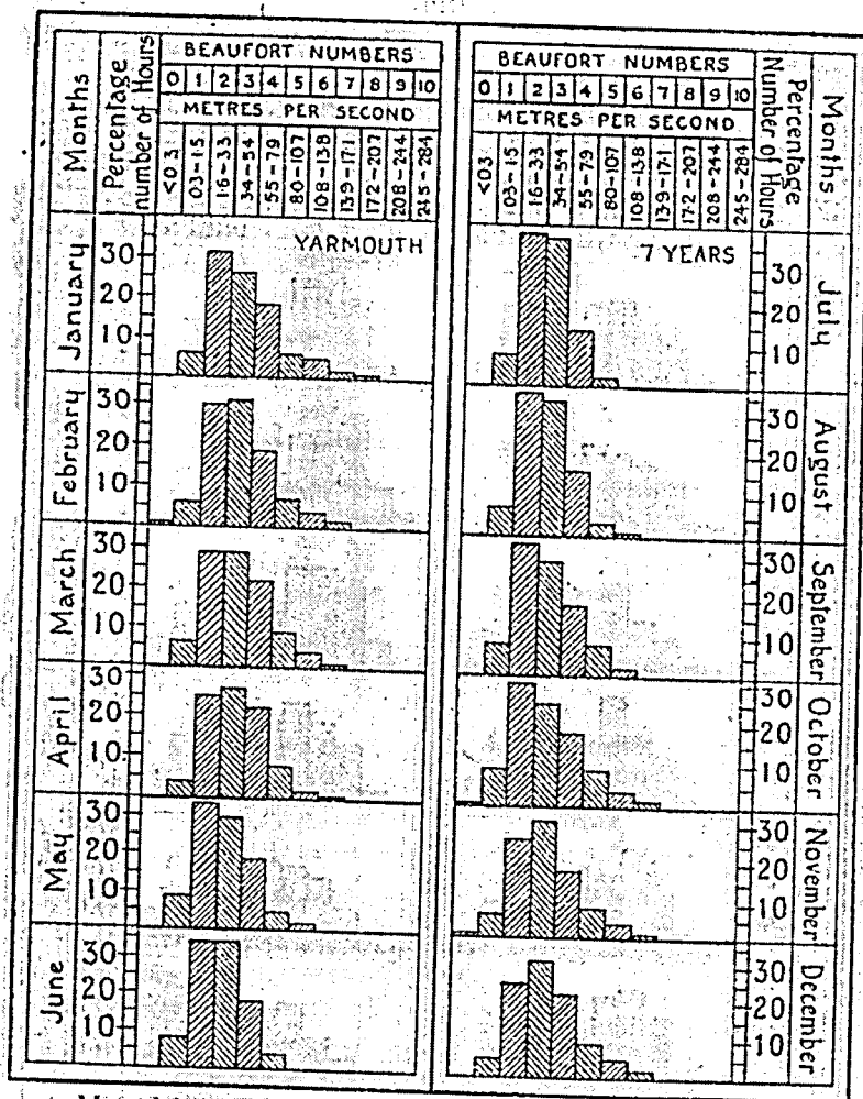
Monthly Average Wind Frequency at Yarmouth.
