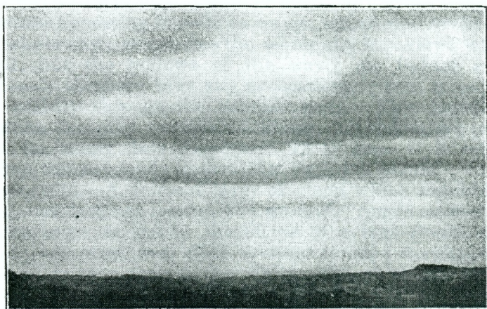
- Strato-Cumulus from below.
