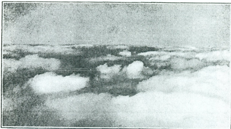
Strato-cumulus from an aeroplane (4,000 feet).
