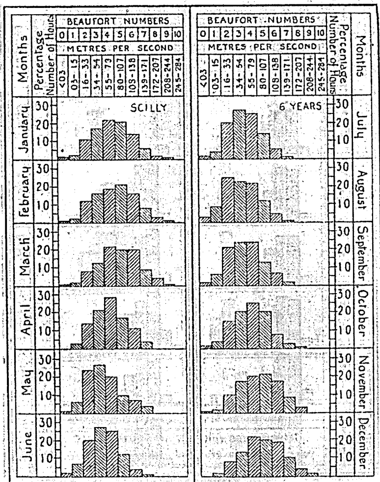
Monthly Average Wind Frequency at Scilly.
