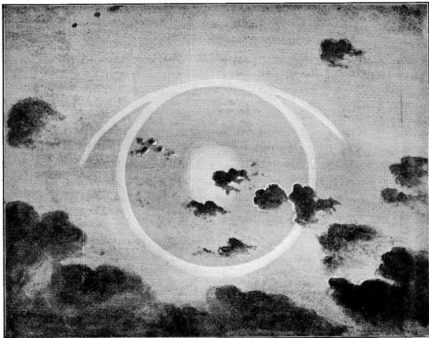
Solar Halo of 22^\circ radius, May 27, 1912. Complete circular halo, with arc of contact. Semi-major axis of the ellipse of which the arc of contact forms a part was about 29^\circ .
