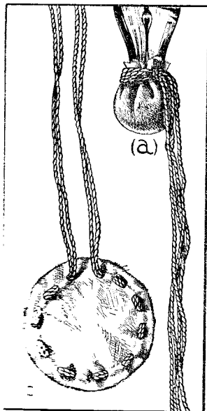
FIG. 14. (a) WET BULB (b) MUSLIN CAP
