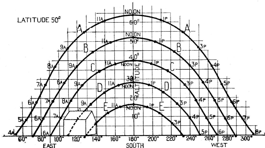
DIAGRAMS SHOWING THE ALTITUDE AND AZIMUTH OF THE SUN AT EACH HOUR (LOCAL APPARENT TIME) FOR PLACES IN LATITUDES 50°, 55°, 60°. (For explanation, see p. 98.)
