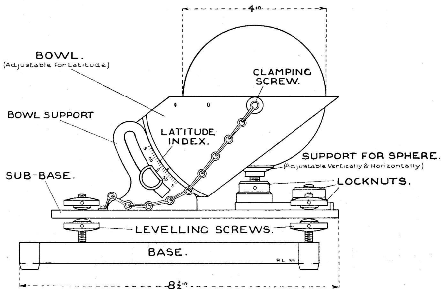
CAMPBELL-STOKES SUNSHINE RECORDER, SIDE VIEW, SHOWING THE ADJUSTMENTS FOR LATITUDE, CONCENTRICITY AND LEVEL.
