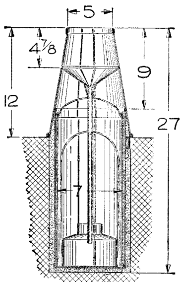
SEATHWAITE RAIN-GAUGE
