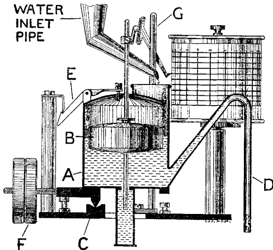
FIG. 29. DINES TILTING SIPHON RAIN-GAUGE.
