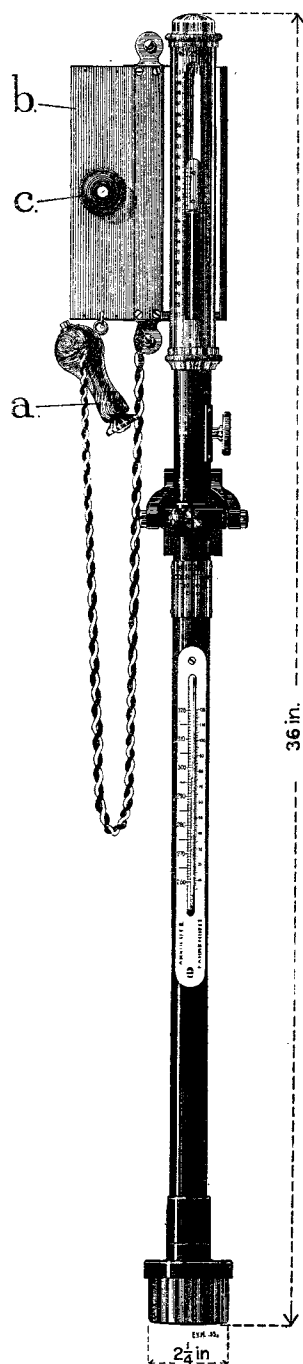
FIG. 4. NEW PATTERN BAROMETER WITH ILLUMINATOR
