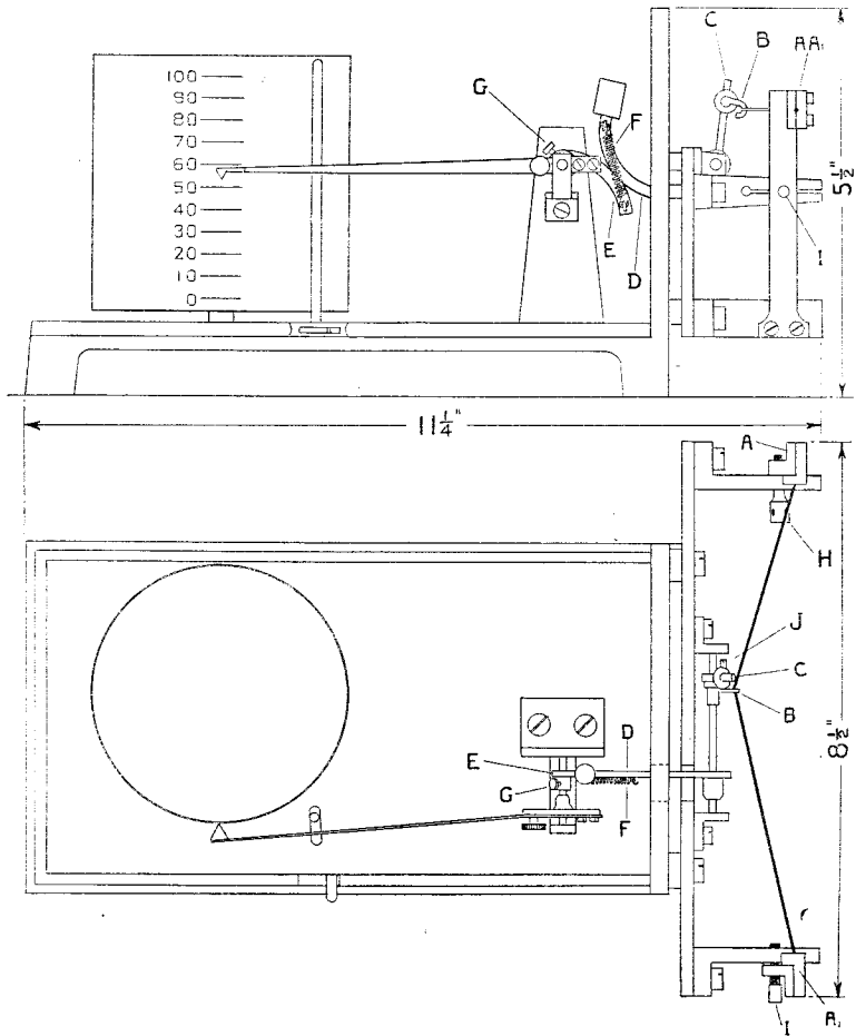
FIG. 25. ELEVATION AND PLAN OF HAIR HYGROGRAPH.
