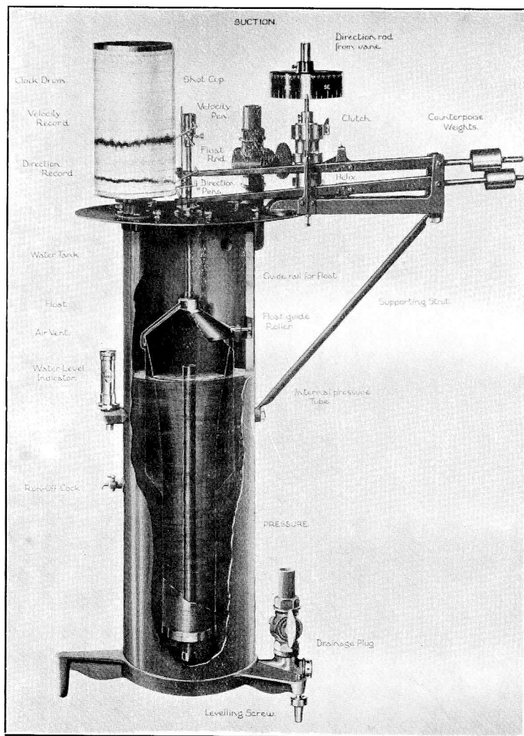
DINES DIRECT RECORDING PRESSURE TUBE ANEMOGRAPH, MK. II
