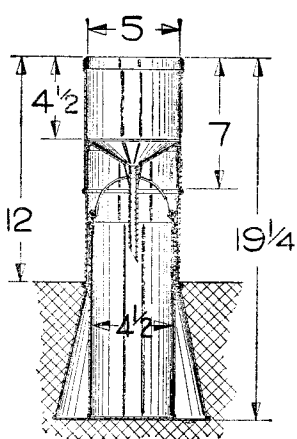
METEOROLOGICAL OFFICE RAIN-GAUGE, Mk. II
