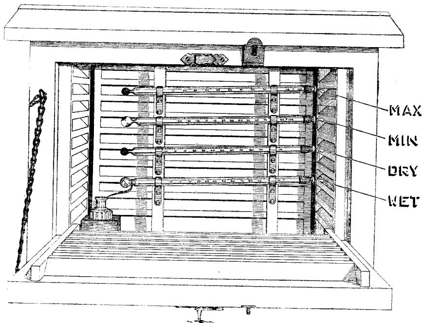
FIG. 11A. BILHAM SCREEN MAXIMUM THERMOMETER
