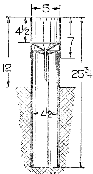
BRADFORD RAIN-GAUGE
