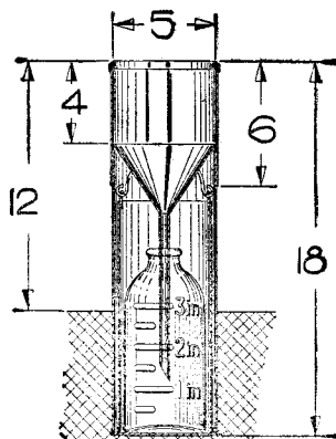
SNOWDON RAIN-GAUGE
