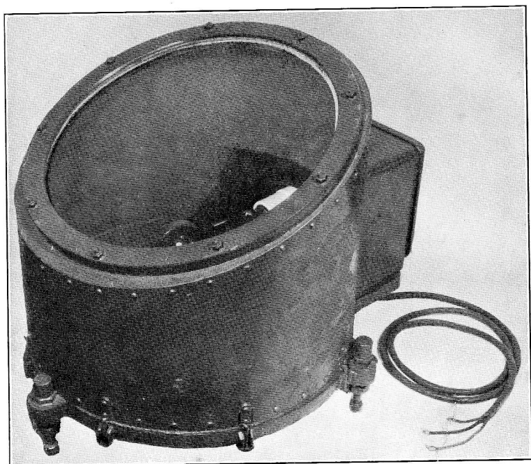
METEOROLOGICAL OFFICE CLOUD SEARCHLIGHT
