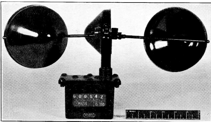
CUP COUNTER ANEMOMETER, MK. II
