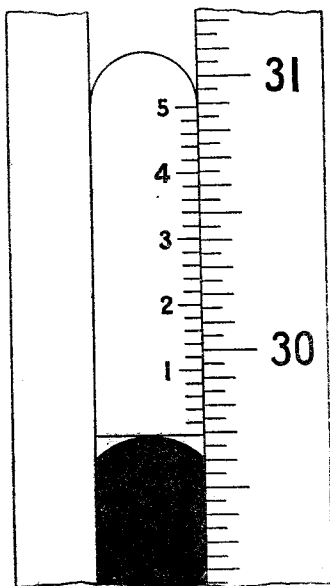
FIG. 7. READING THE SCALE (Inch Graduations.)
