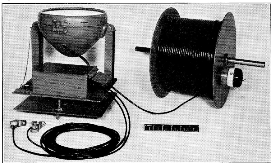
METEOROLOGICAL OFFICE PORTABLE CLOUD SEARCHLIGHT
