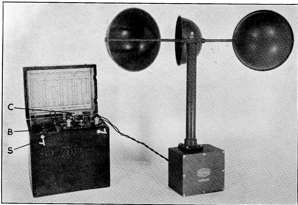
CUP CONTACT ANEMOMETER, MK. I, AND PORTABLE RECEIVER (B = Battery, C = Buzzer, S = Switch.)
