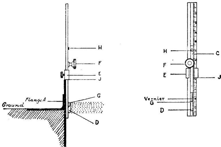
FIG. 23B. HOOK-GAUGE
