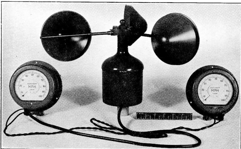
CUP GENERATOR ANEMOMETER, MK. IA
