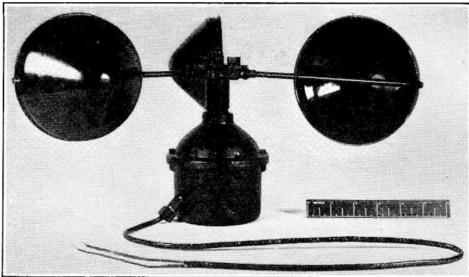
CUP CONTACT ANEMOMETER, MK. II
