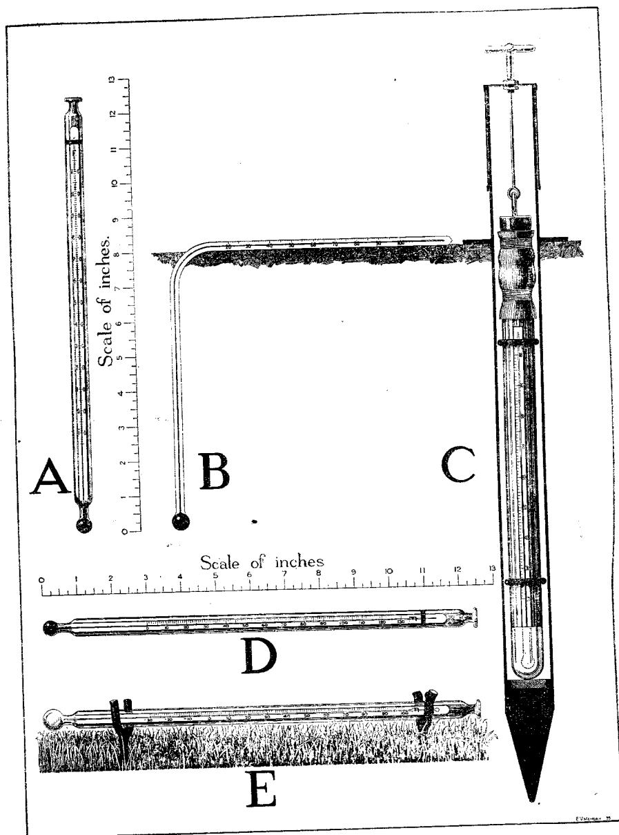
FIG. 10. STANDARD PATTERNS OF THERMOMETERS
