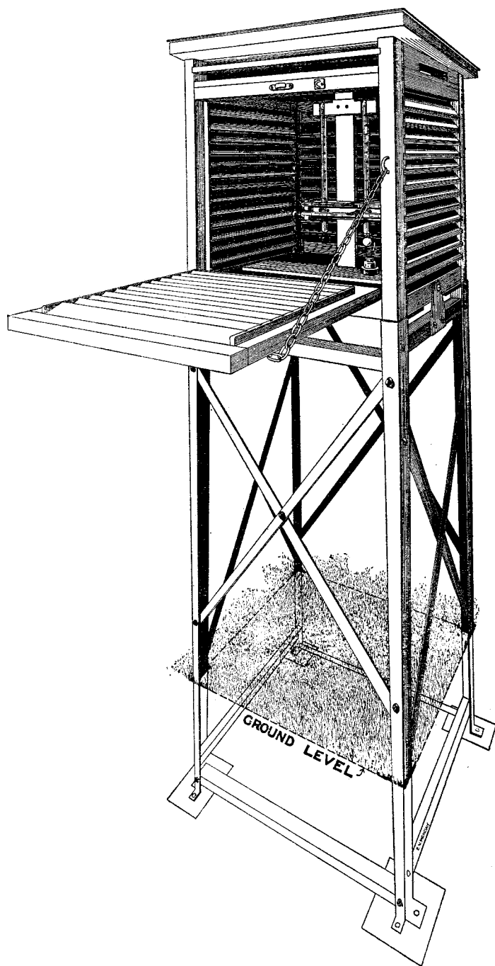
FIG. 11. STEVENSON SCREEN WITH SHEATHED THERMOMETERS AND STEEL STAND
