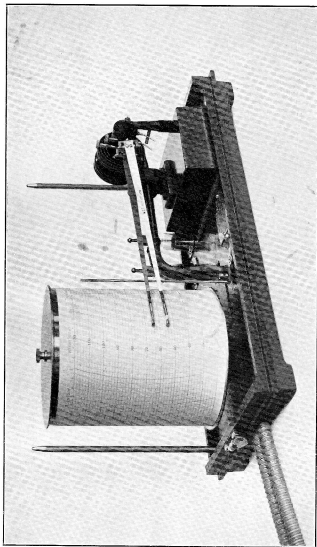
DISTANT-READING THERMOGRAPH.
