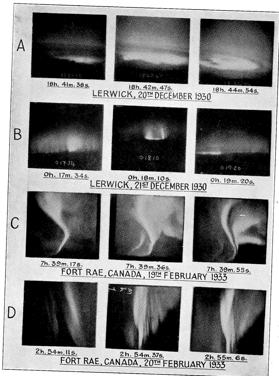
PHOTOGRAPHS OF THE AURORA (For description see p. 72.)
