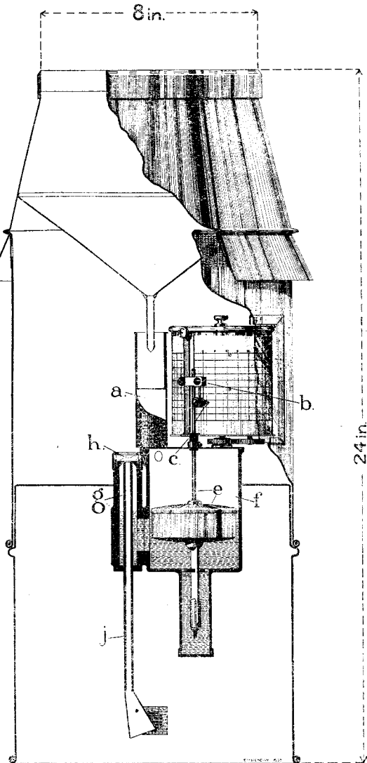
FIG. 30. NATURAL SIPHON RECORDING RAIN-GAUGE.
