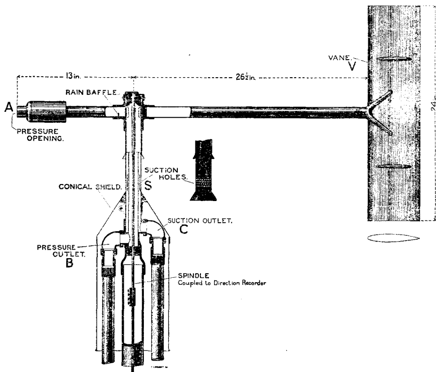
FIG. 26. HEAD OF DINES ANEMOGRAPH (Mark II).
