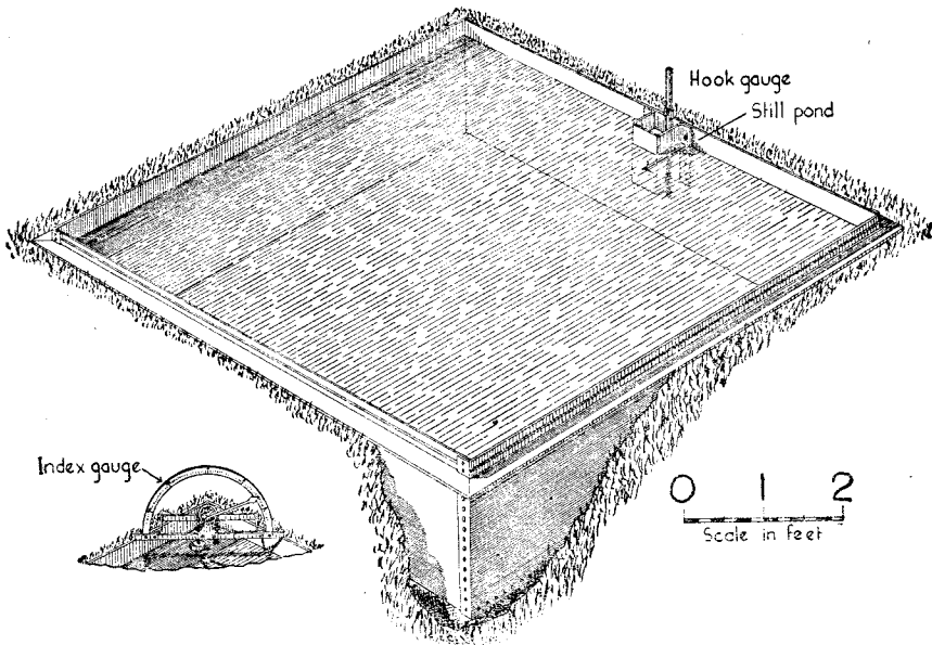
FIG. 23A. EVAPORATION TANK—BRITISH STANDARD
