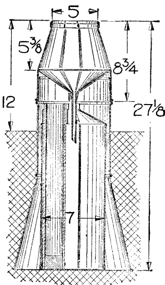
OCTAPENT RAIN-GAUGE
