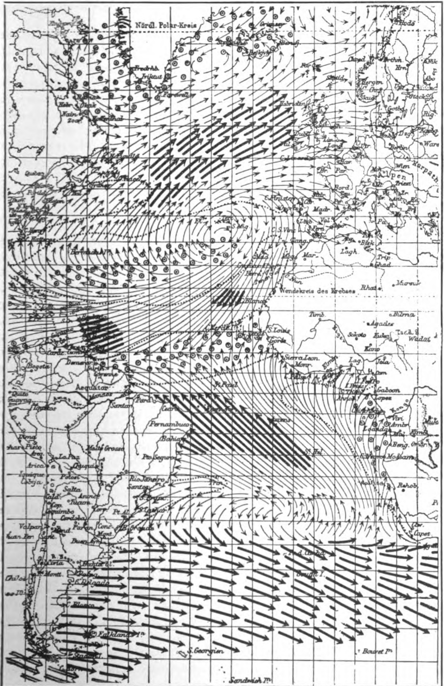
FIG. 41. — GENERAL WINDS OF THE ATLANTIC FOR JULY. (From the Atlantic Sailing Handbook of the German Naval Observatory.)
