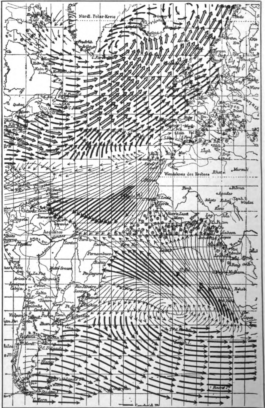
FIG. 40. — GENERAL WINDS OF THE ATLANTIC FOR JANUARY.
