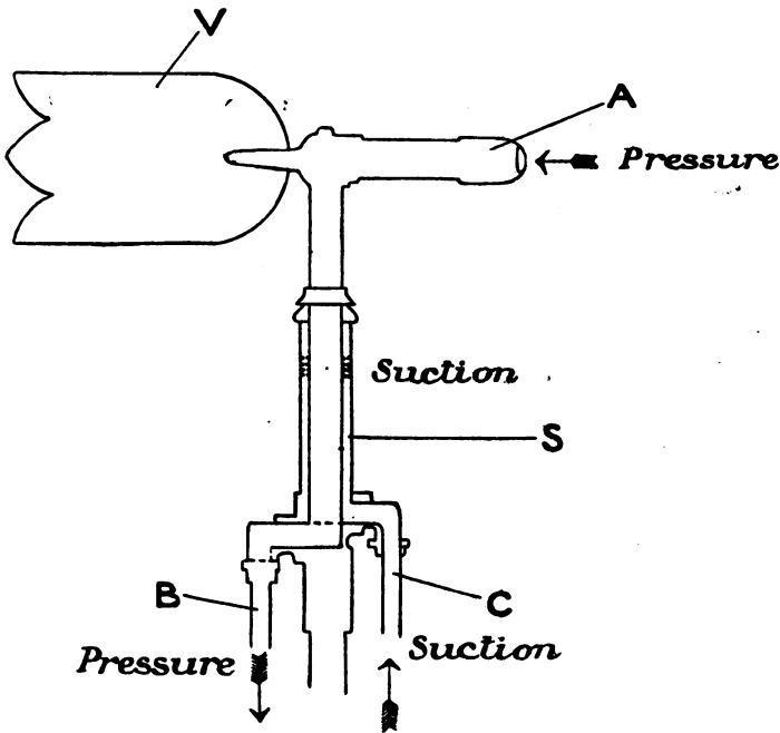
FIG. 1.—Head of Dines Pressure Tube Anemometer.
