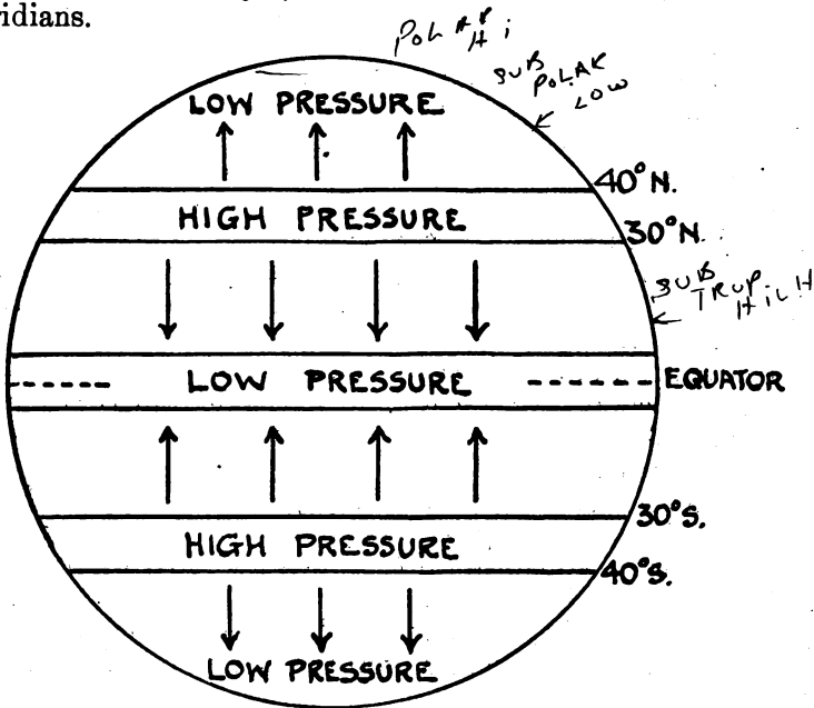
FIG. 4.—General Scheme of Pressure over the Earth with Winds as they would be if the Earth did not rotate.
