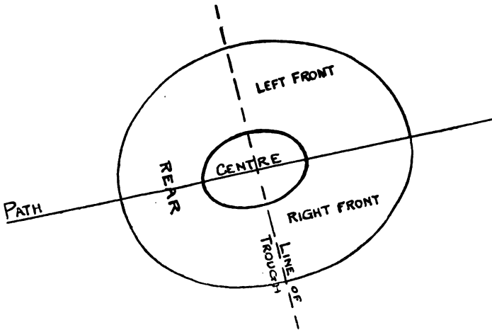
FIG. 11.—NOMENCLATURE OF A DEPRESSION.
