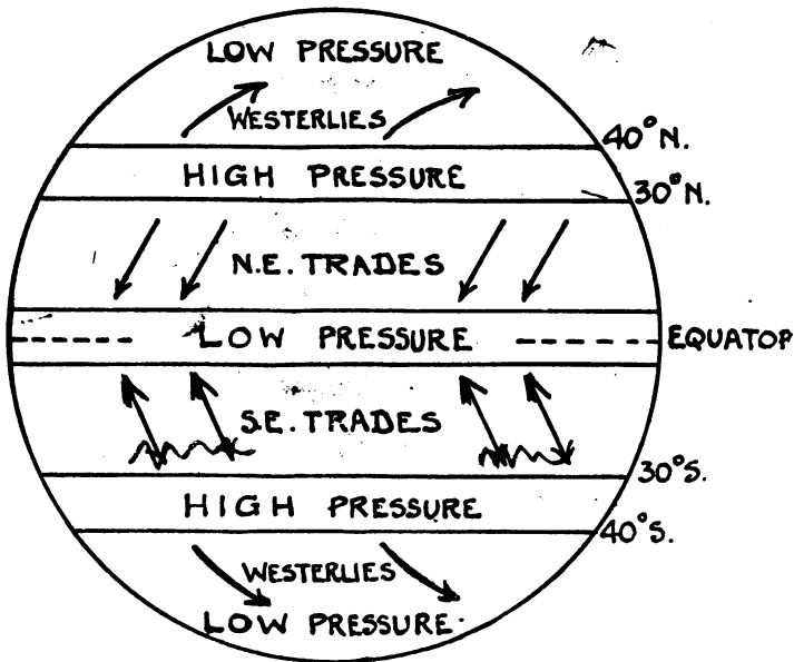
FIG. 5.—Scheme of Winds as they actually blow taking into account the Rotation of the Earth.
