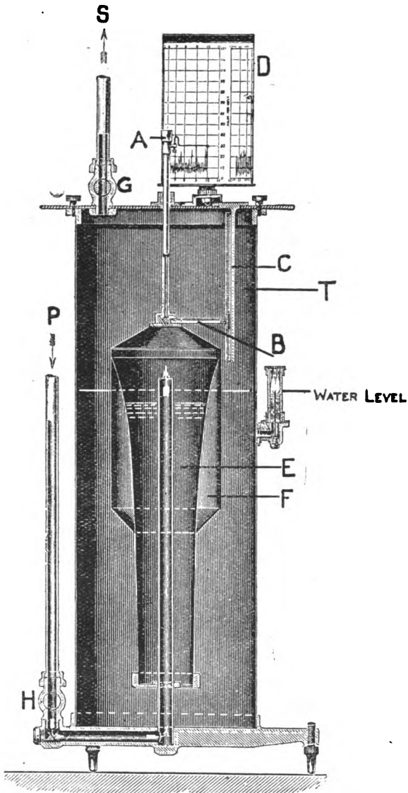
FIG. 2.—Recording Apparatus of Dines Pressure Tube Anemometer.
