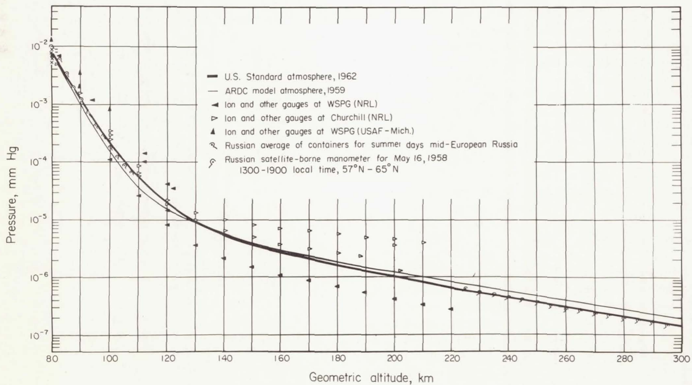
FIGURE II.2.2(c).—Pressures of U.S. Standard Atmosphere, 1962 compared with ARDC Model Atmosphere, 1959 and with available data.
