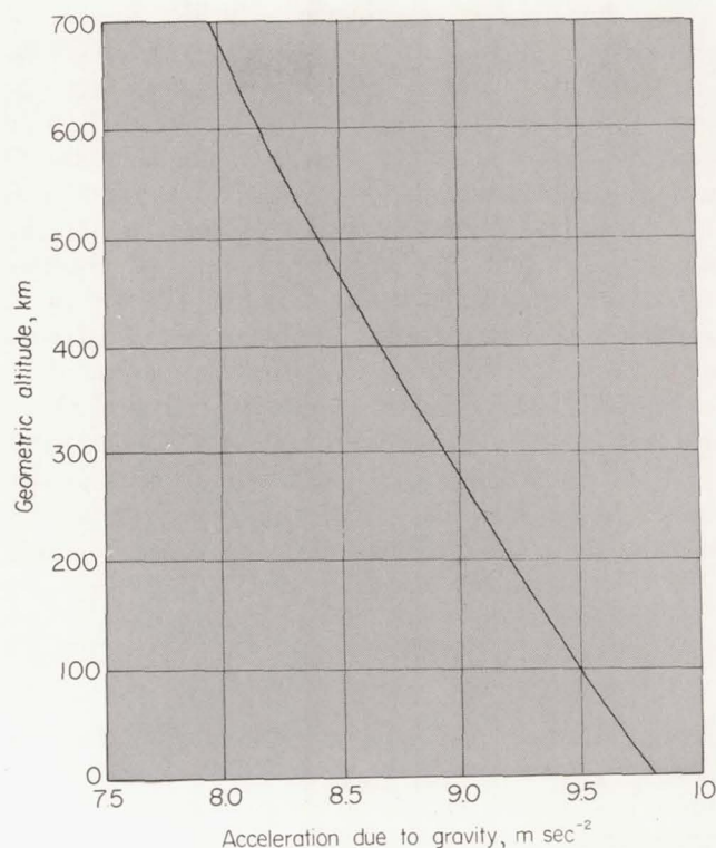
FIGURE I.2.4(b).—Acceleration due to gravity g as a function of geometric altitude Z .
