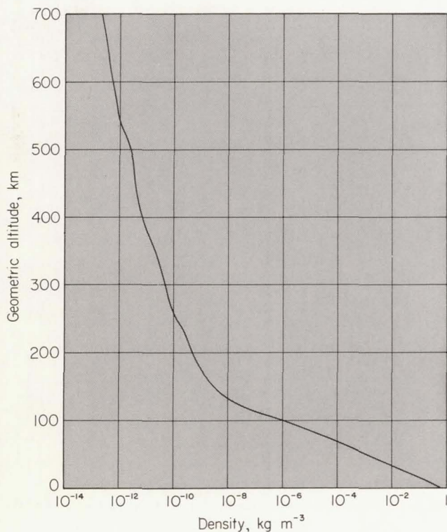
FIGURE I.2.11.—Density \rho as a function of geometric altitude Z .
