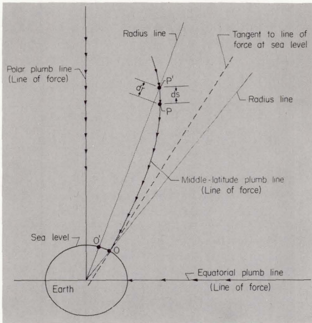
FIGURE I.2.4(a).—Relationships between various heights.
