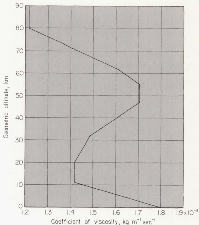
FIGURE I.3.8.—Coefficient of viscosity \mu as a function of geometric altitude Z .
