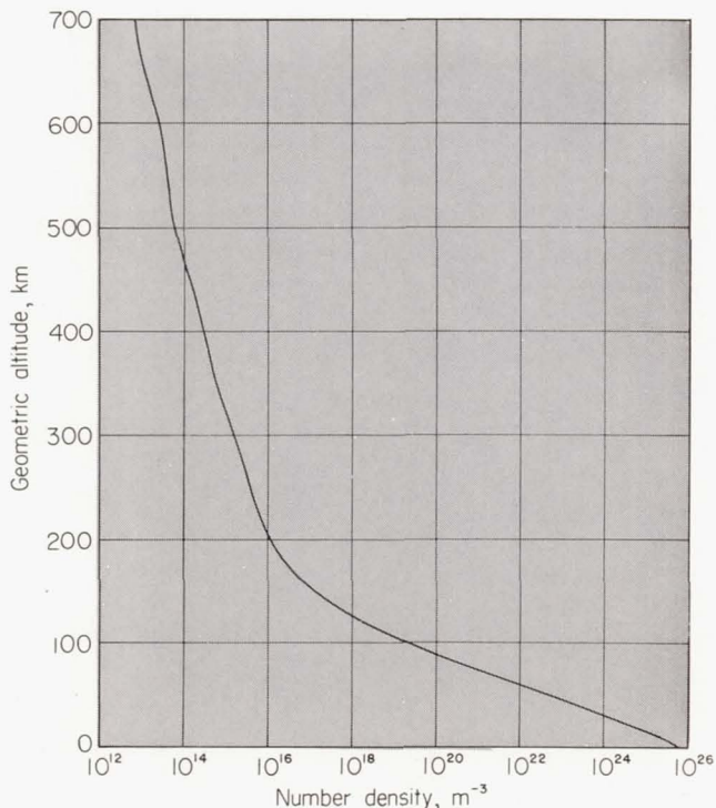
FIGURE I.3.3.—Number density n as a function of geometric altitude Z .
