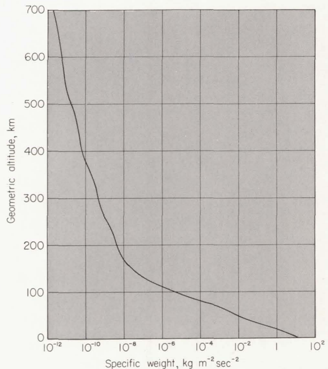
FIGURE I.3.1.—Specific weight \omega as a function of geometric altitude Z .
