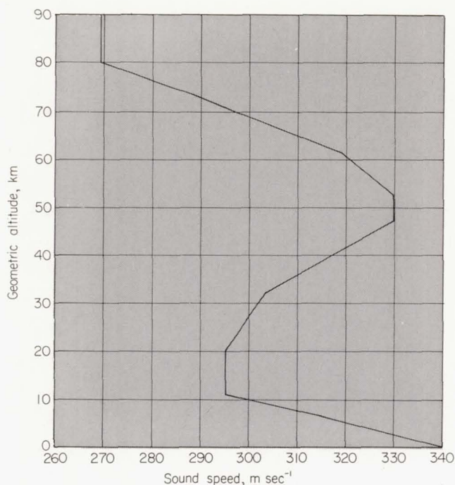
FIGURE I.3.7.—Sound speed C_s as a function of geometric altitude Z .
