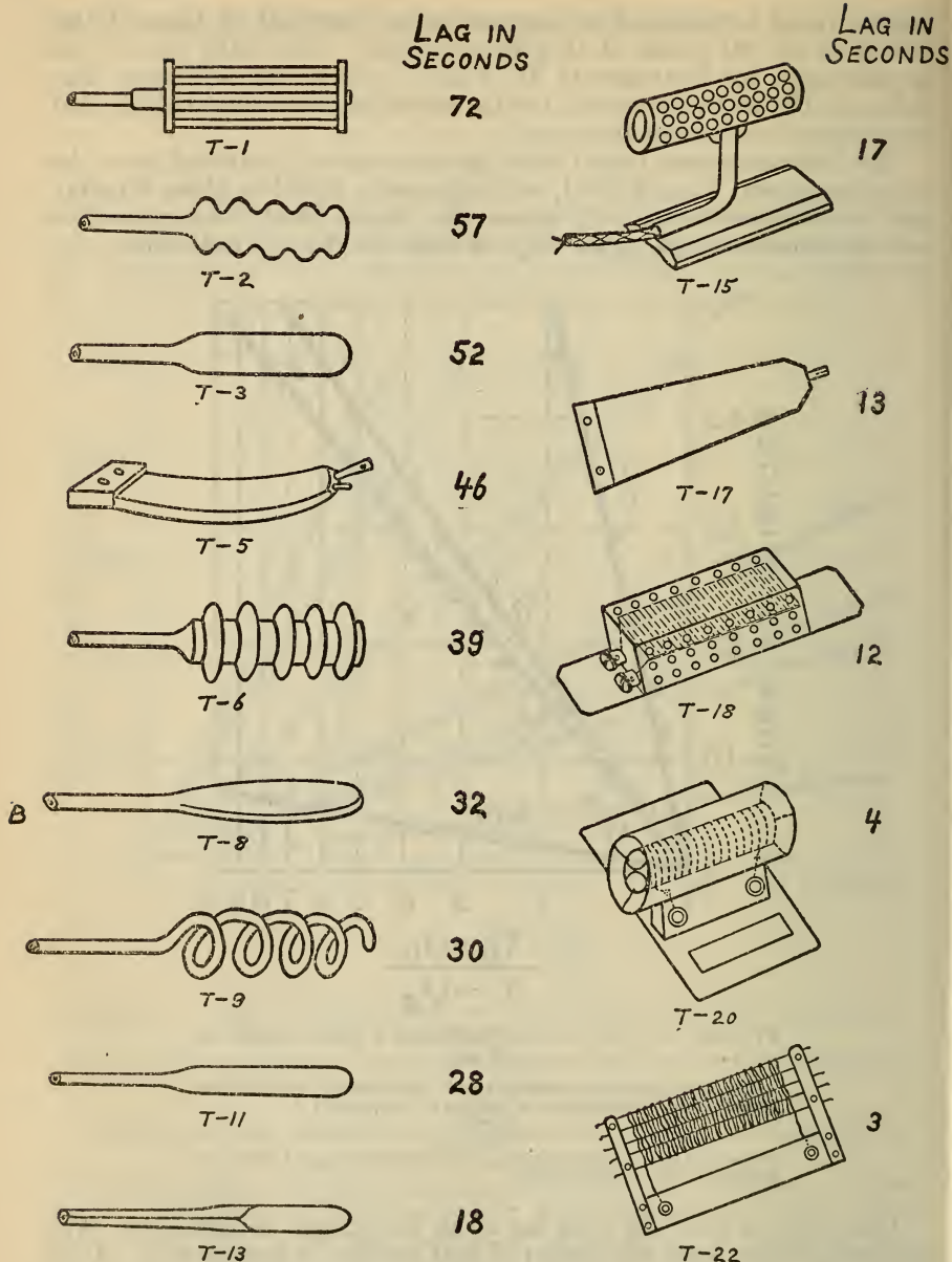
FIGURE 3.—Sketches of the temperature elements of a number of thermometers and thermographs
