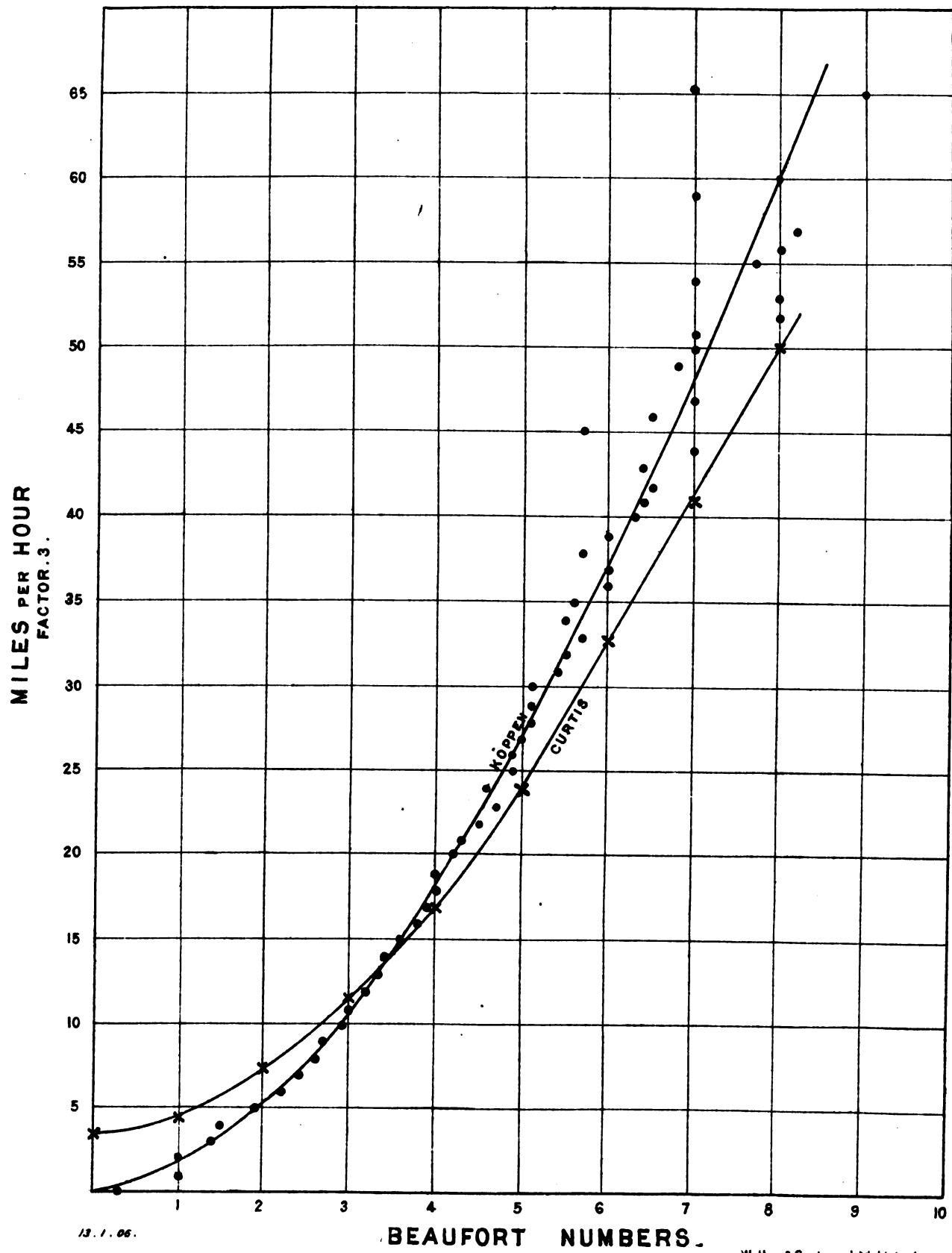
Figure 1. BEAUFORT NUMBERS AND MILES (NOMINAL) PER HOUR.
