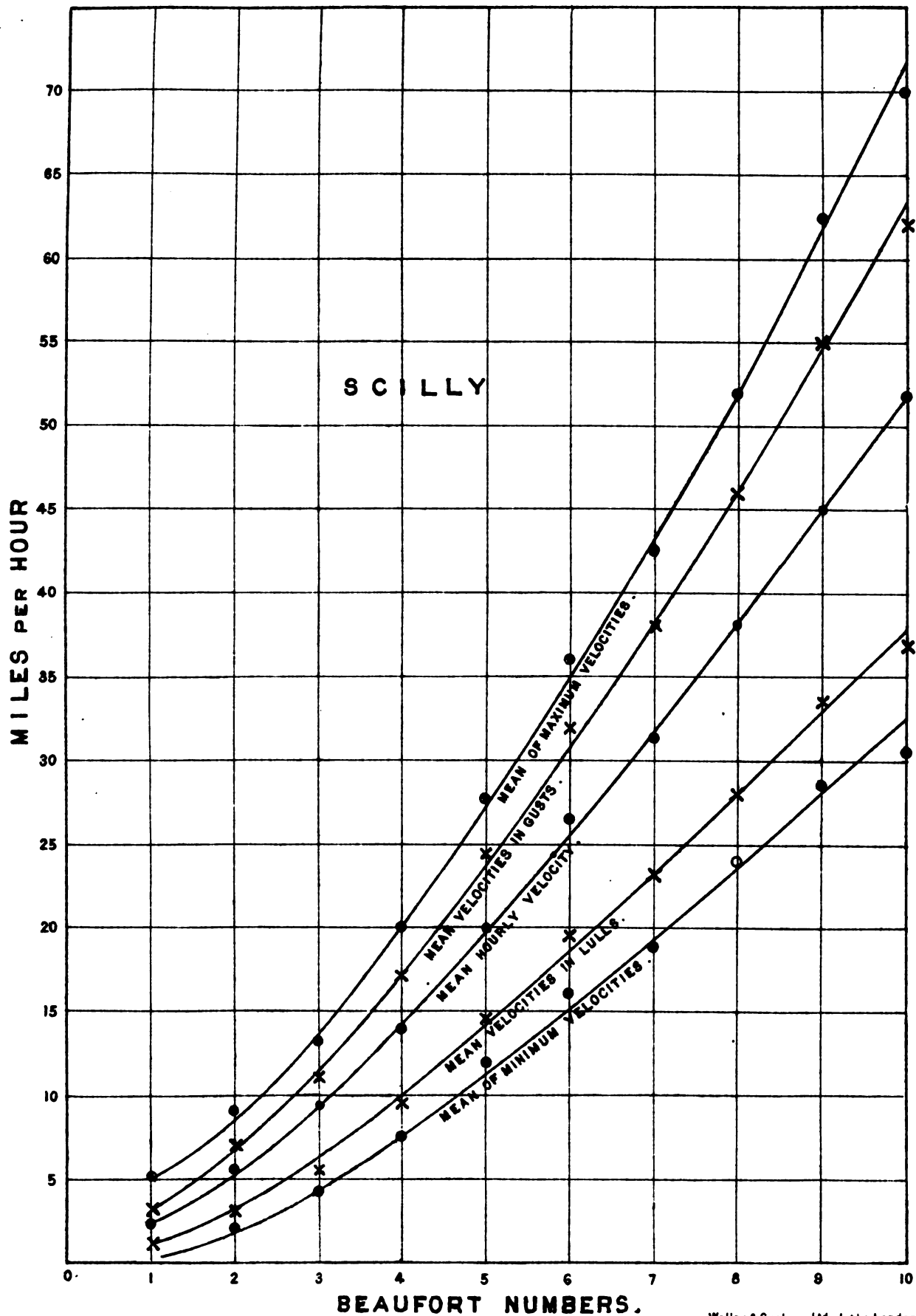
Figure 7. AVERAGE RELATION BETWEEN THE BEAUFORT NUMBERS AND THE SEVERAL CHARACTERISTICS OF CORRESPONDING WINDS.
