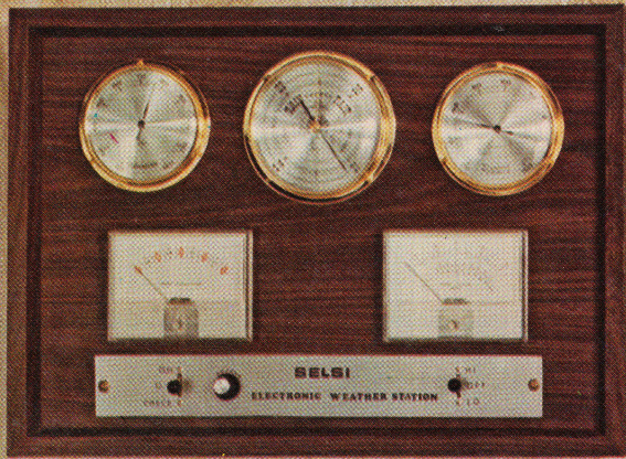
(A) ELECTRONIC WEATHER STATION. Precision instrument panel registers weather conditions on one panel. Complete with roof transmitter. Lead in cord, measures wind direction and speed. Console 17"x12"x3" can be hung on wall. Contains barometer, thermometer, hygrometer. Operates on flashlight battery not supplied. Shpg. wt. 15 lbs. 840
