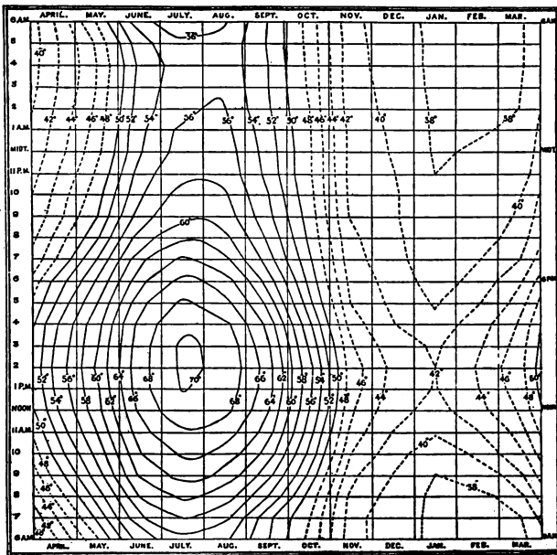
Chrono-isothermal Diagram representing the Monthly Mean Temperature at Greenwich, for every hour of the day through the range of years 1849 to 1868.
