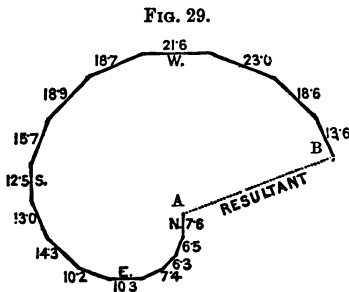
Diagram of the mean hourly Velocity of the Wind at Liverpool in January (1852-63).
