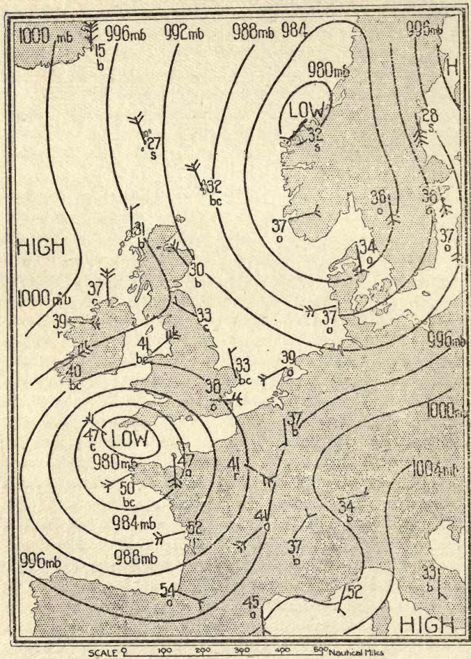
Secondary Depression. 7am, Thursday, 1st January, 1920.
