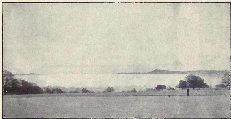
FIG. 20—VALLEY FILLED WITH FOG, 300 FEET DEEP, IN EARLY MORNING AFTER STILL NIGHT
