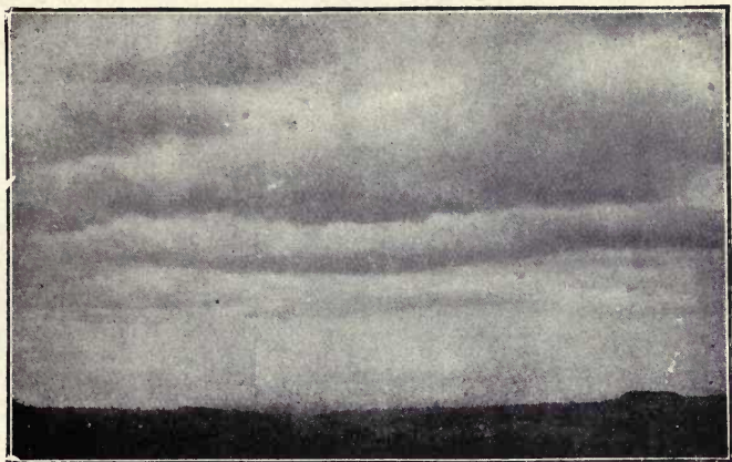
FIG. 17—STRATO-CUMULUS FROM BELOW
