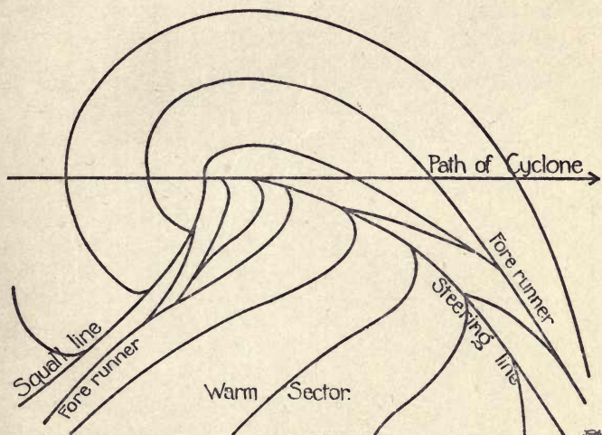
Lines of Flow in a Moving Cyclone after Bjerknes.
