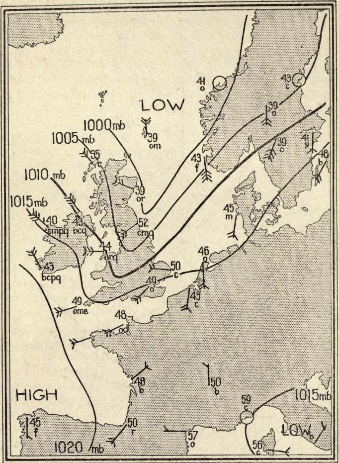
"V" Shaped Depression 7 a.m. Tuesday, 20th April, 1915.
