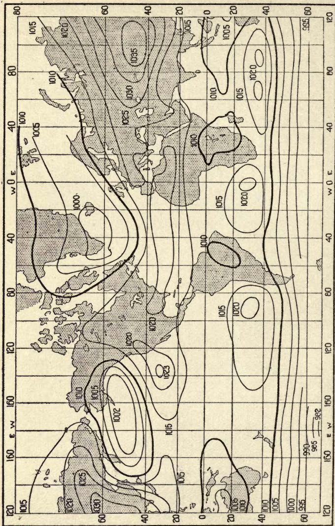
Average Isobars for the World for January, at Sea Level.
