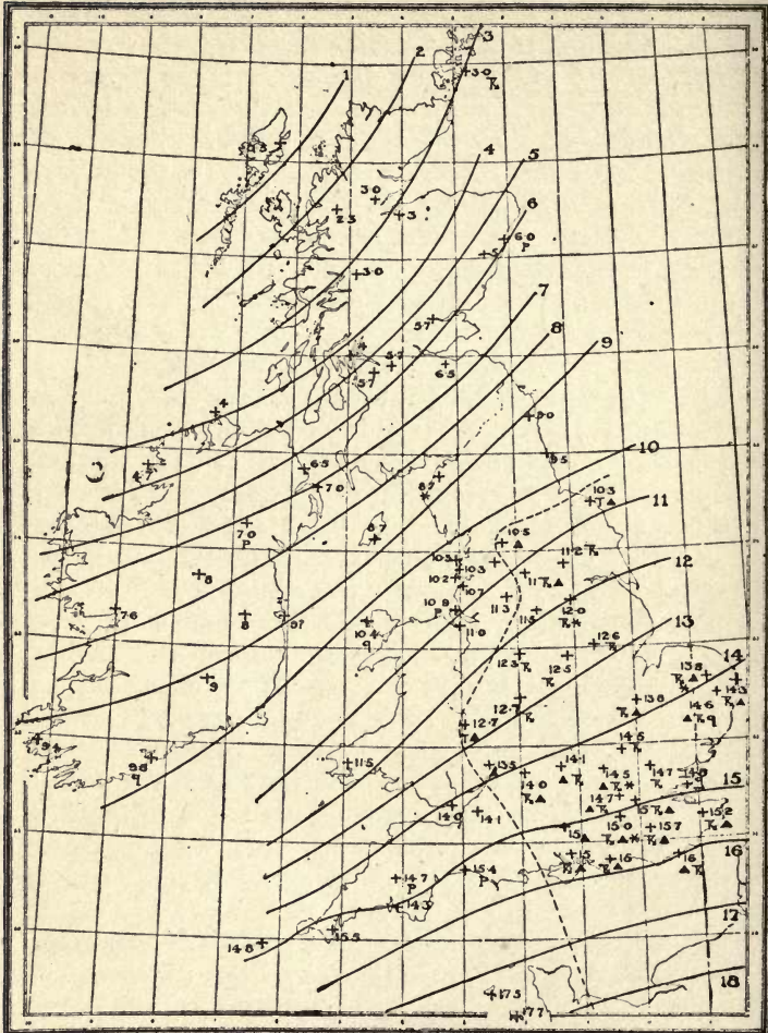
FIG. 36—ISOCRONOUS LINES FOR FEBRUARY 8TH, 1906
