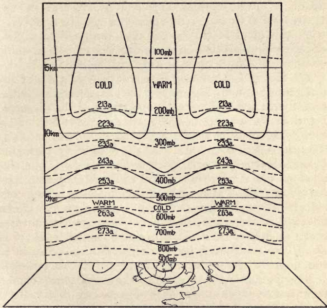
DISTRIBUTION OF TEMPERATURE AND PRESSURE IN CYCLONES AND ANTICYCLONES Mean Values after W.H. Dines.
