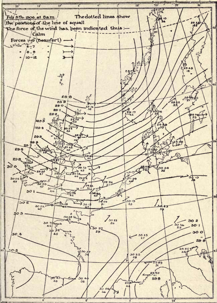
FIG. 37—ISOBARS AND WIND ON FEBRUARY 8TH, 1906, AT 8 A.M.
