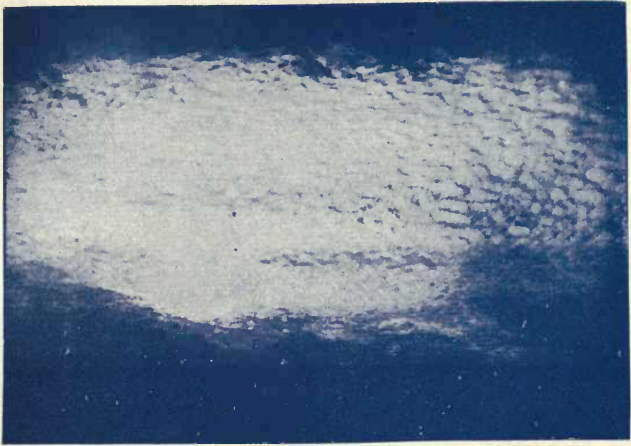
FIG. 15—CIRRO-CUMULUS BECOMING ALTO-CUMULUS 12 H. 5 M.
