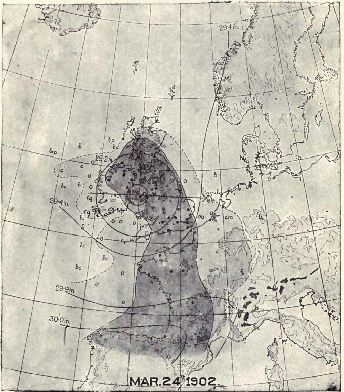
FIG. 4—DISTRIBUTION OF RAIN AND CLOUD IN CYCLONE
