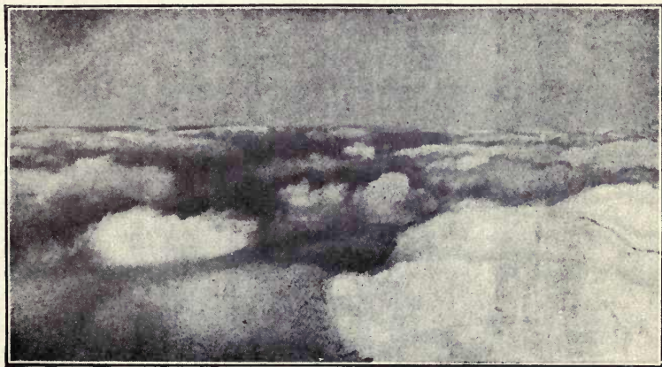
FIG. 18—STRATO-CUMULUS FROM AN AEROPLANE (4,000 FEET)
