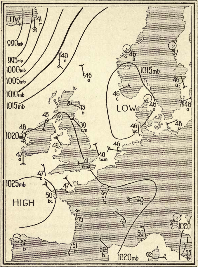
Anticyclonic Wedge, 7am, Friday, 19th, October, 1917.
