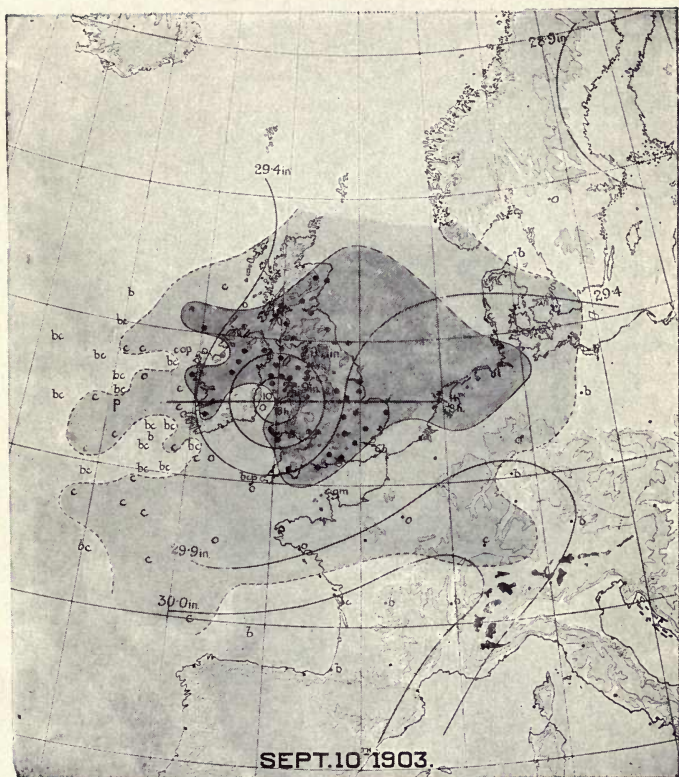
FIG. 5—DISTRIBUTION OF RAIN AND CLOUD IN CYCLONE
