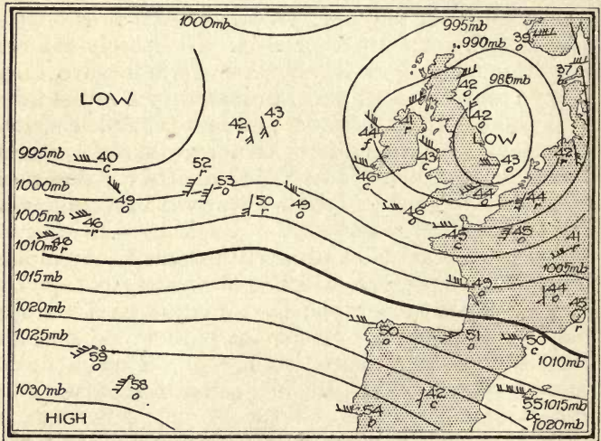
SCALE 0 1 2 3 4 Nautical Miles Westerly Type, 7am, Friday, 22nd March, 1912
