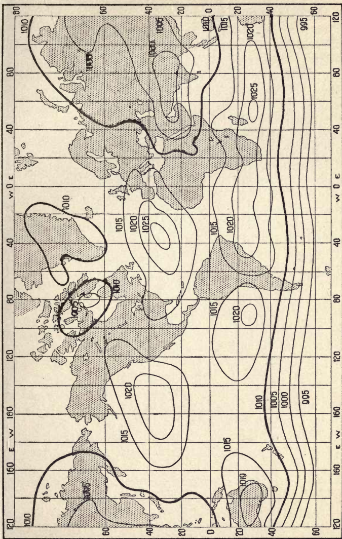
Average isobars for the World for July at Sea Level.
