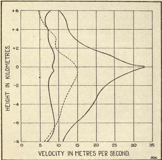
Decrease of wind in the Stratosphere.
