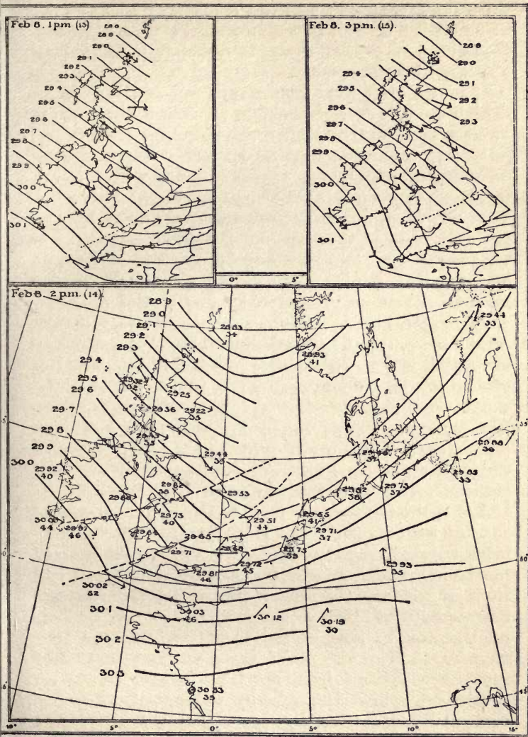
FIG. 38—ISOBARS AND WIND ON FEBRUARY 8TH, 1906, AT 1 P.M., 2 P.M., AND 3 P.M.
