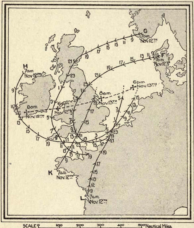
Trajectories of November 11th, 1901.
