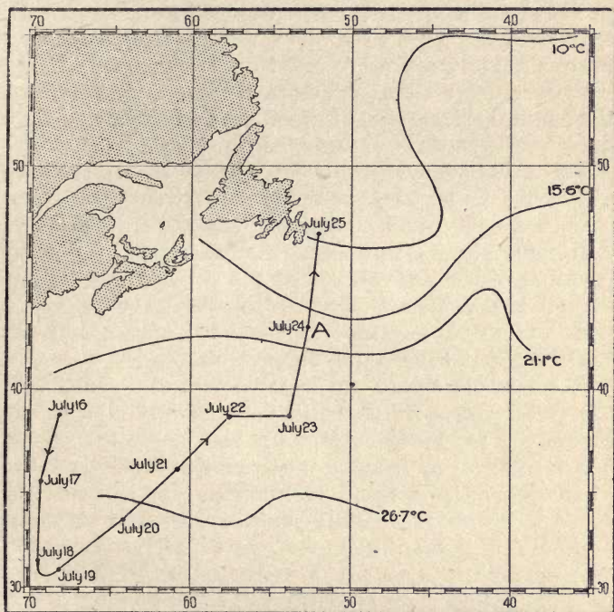
Trajectories of Air over the Atlantic, — July, 1913.
