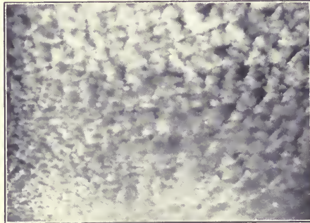
Fig. 80. Alto-cumulus.
