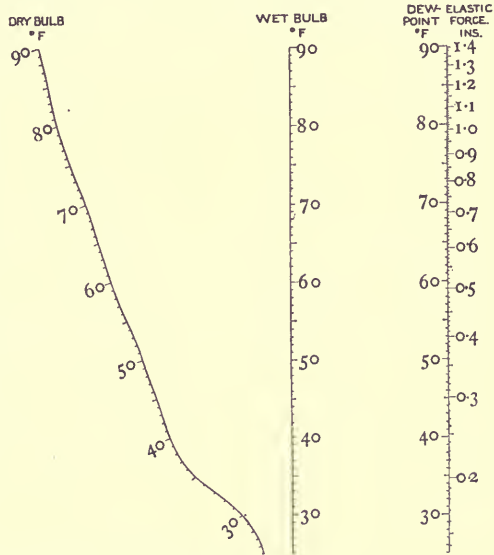
Fig. 110. Nomogram for the calculation of dew-point and vapour-pressure (J. Ball).
