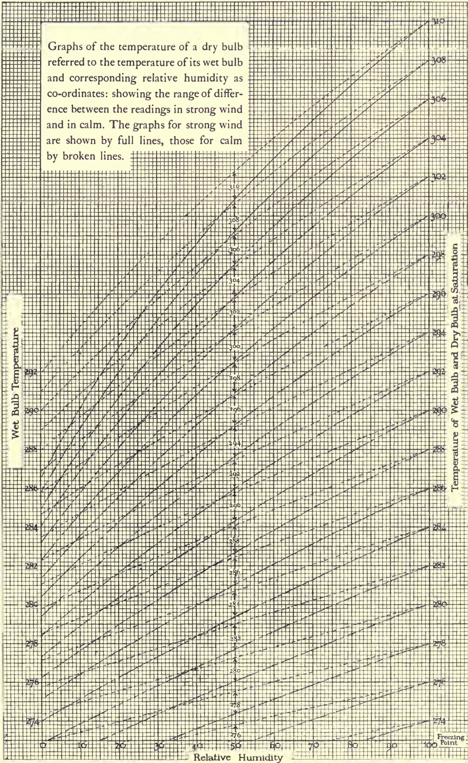
Fig. 18. Diagram for obtaining the relative humidity from readings of the wet and dry bulb thermometers in strong wind and calm.
