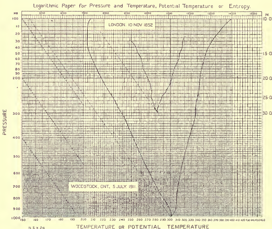
Fig. 105. Examples of graphs of soundings of the atmosphere referred to pressure-temperature and pressure-potential-temperature respectively (1) for an ascent in a manned balloon by J. Welsh at Vauxhall in 1852, and (2) for a sounding with a registering balloon in Canada in 1911. The two graphs for each occasion meet on the line of standard pressure. The observations of pressure in (1) are in inches and in (2) millibars; both are plotted direct on to the paper without conversion as curves in full line. The faint straight pecked lines are adiabatic lines for dry air.
