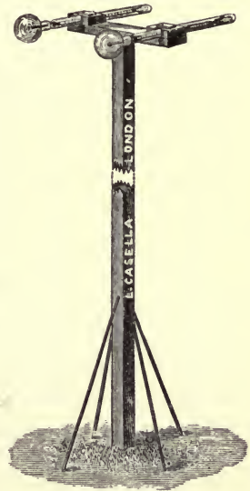
FIG. 11.—SOLAR RADIATION THERMOMETER STAND.
