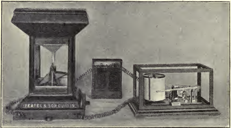
FIG. 63.—YEATES'S ELECTRICAL SELF-REGISTERING RAIN-GAUGE.
