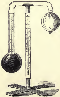
FIG. 46.—DANIELL'S HYGROMETER.
