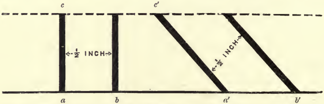
FIG. 94.—DIAGRAM ILLUSTRATING THE EFFECT OF THE PERPENDICULAR AND THE OBLIQUE FALLING OF THE SUN'S RAYS.
