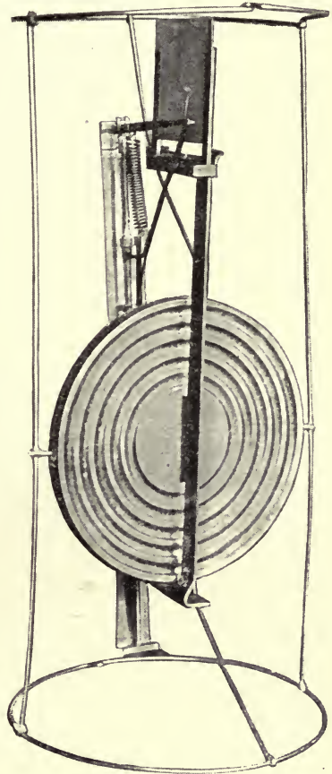
FIG. 90.—DINES'S BALLOON METEOROGRAPH.
