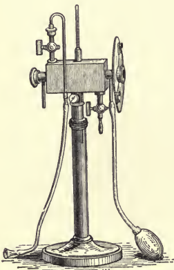
FIG. 51.—CROVA'S HYGROMETER.
