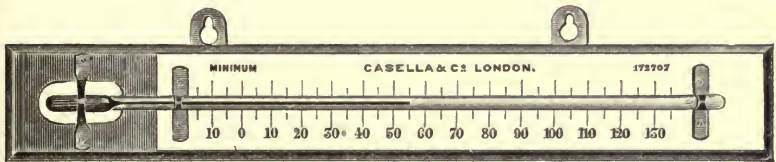
FIG. 5.—RUTHERFORD'S MINIMUM THERMOMETER, FILLED WITH PURE ALCOHOL FOR ORDINARY REGISTRATION, ENGINE-DIVIDED ON THE STEM.
