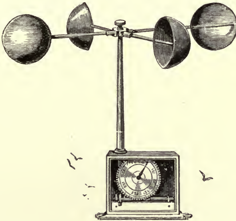
FIG. 76.—ROBINSON'S ANEMOMETER.
