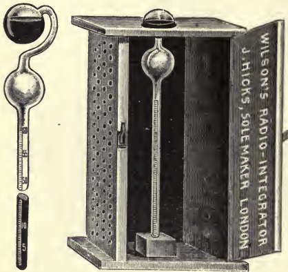
FIG. 13.—WILSON'S PATENT RADIO-INTEGRATOR.
