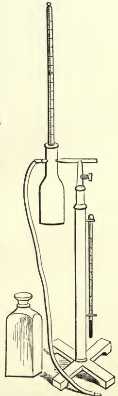
FIG. 47.—REGNAULT'S HYGROMETER.
