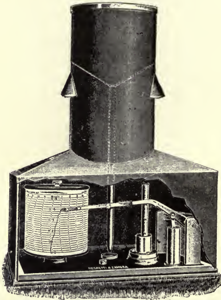
FIG. 67.—NEGRETTI AND ZAMBRA'S HYETOGRAPH (UPPER PART).
