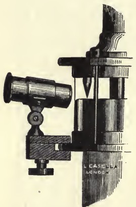
FIG. 24.—WALLIS'S ARRANGEMENT FOR ADJUSTING THE IVORY POINT.
