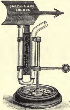
FIG. 75.—LIND'S ANEMOMETER.
