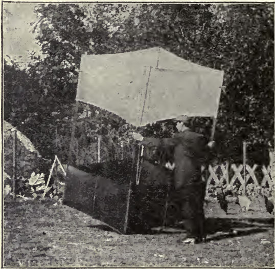
FIG. 89.—KITE CONSISTING OF TWO STRIPS OF MATERIAL STRETCHED INTO QUADRANGULAR SAILS ON A LOZENGE-SHAPED PLAN UPON FOUR TRANSVERSE BARS KEPT APART BY TWO PAIRS OF CROSS-STRUTS.
