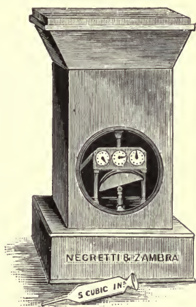
FIG. 62.—CROSLY'S SELF-REGISTERING RAIN-GAUGE.
