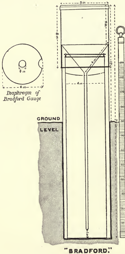
FIG. 61.—BRADFORD RAIN-GAUGE.
