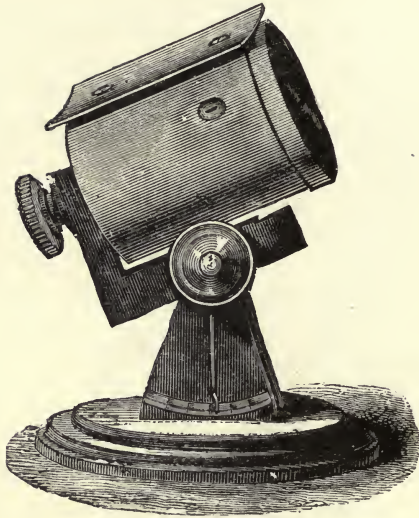
FIG. 19.—JORDAN PHOTOGRAPHIC SUNSHINE RECORDER.
