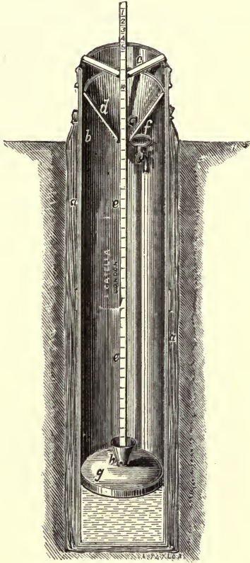
FIG. 60.—MOUNTAIN RAIN-GAUGE.
