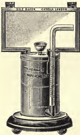
FIG. 45.—PICKERING'S STANDARD EVAPORIMETER.
