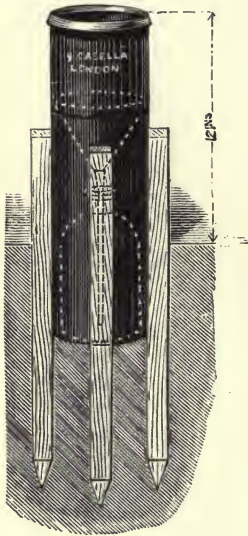
FIG. 59.—SNOWDON RAIN-GAUGE.
