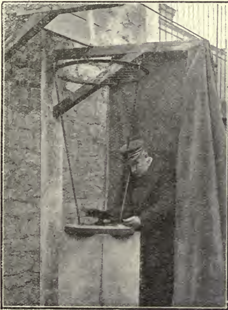
FIG. 55.—BESSON'S ZENITH NEPHOSCOPE.
