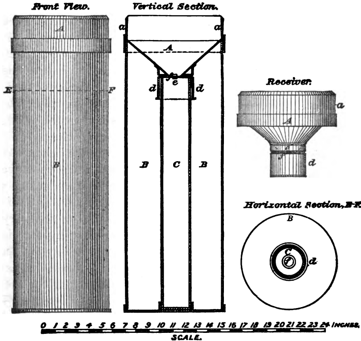
FIGURE 14. Rain-gauge.
