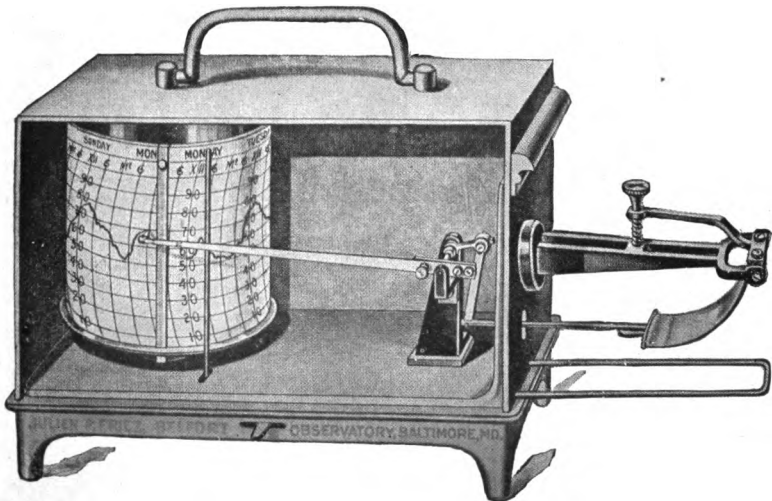
FIGURE 16. Richard's Thermograph.
