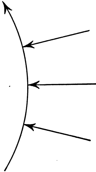
FIGURE 65. Path of winds in frictionless flow under a converging force.
