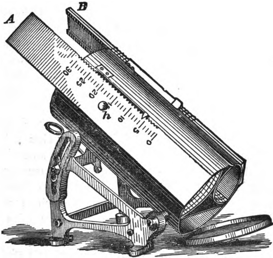
FIGURE 19. Photographic Sunshine Recorder.
