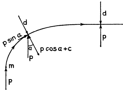
FIGURE 64. Deflection and path of winds in frictionless flow under a force of constant magnitude and constant geographic direction.
