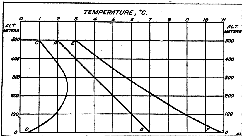
FIGURE 22. Examples of different states of equilibrium: AB, adiabatic gradient for dry air (neutral equilibrium); CD, temperature inversion (stable equilibrium); and EF, superadiabatic gradient (unstable equilibrium).
