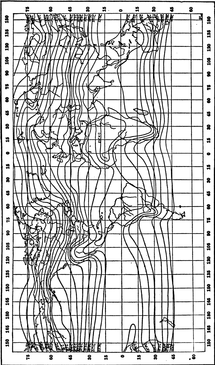
FIGURE 33. Average annual isotherms, °C (after Buchan).
