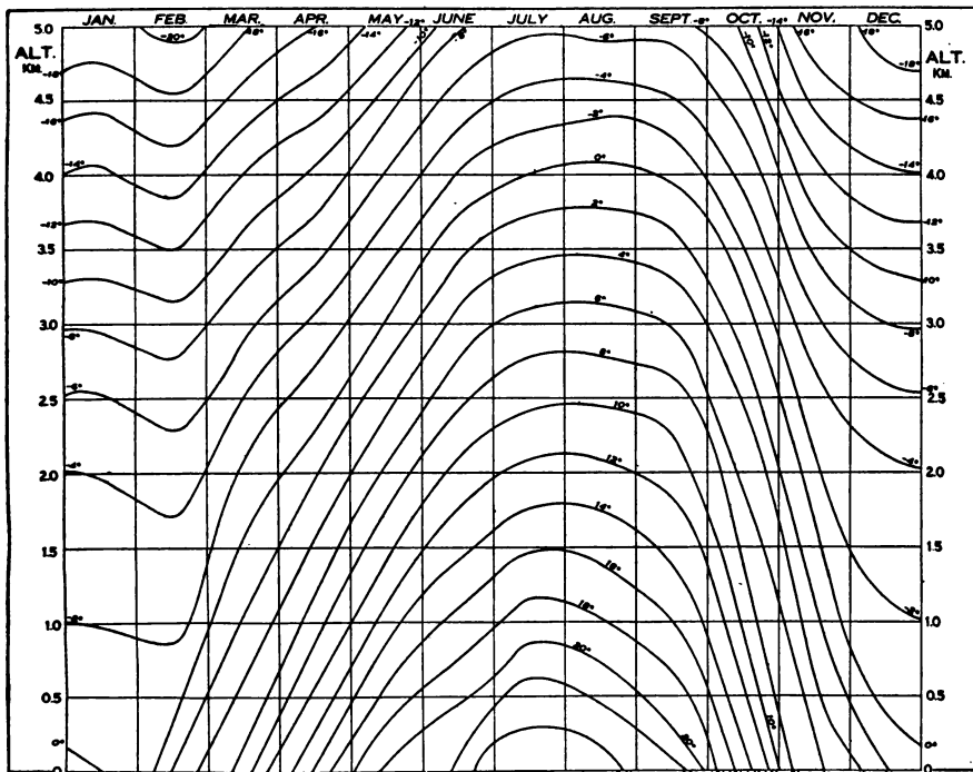
FIGURE 24. Mean annual march of free air temperatures, °C, above Mount Weather, Va., altitude 526 meters. (Lines extended to sea level by extrapolation.)
