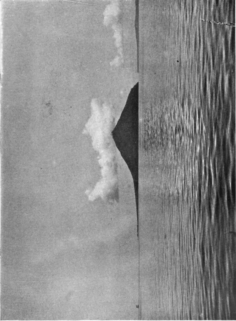
FIGURE 57. Cumulus over island—Krakatoa. (E. E. Barnard, photo.)
