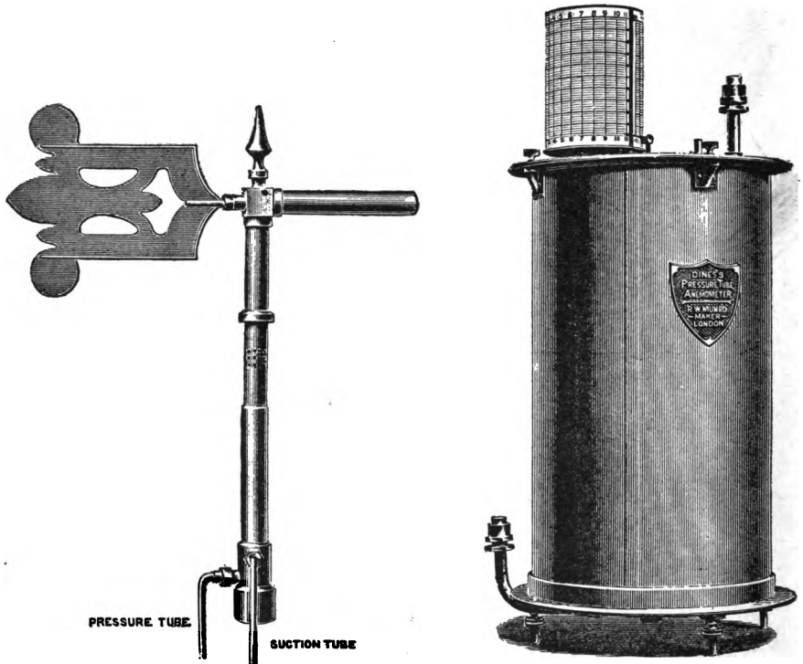
FIGURE 10. Dines' Pressure-tube Anemograph.
