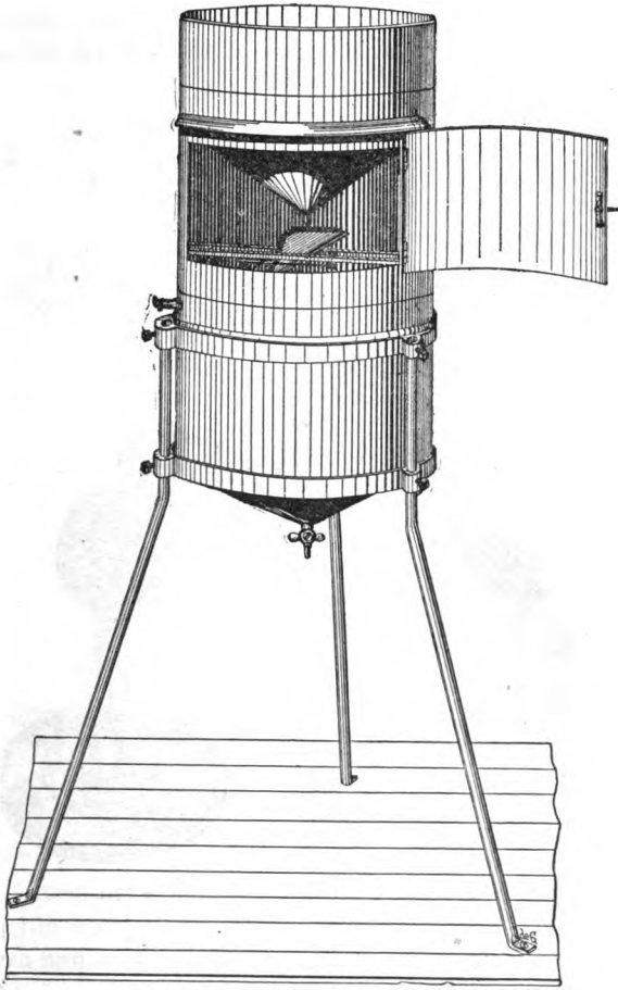
FIGURE 17. Tipping-bucket Rain-gauge.
