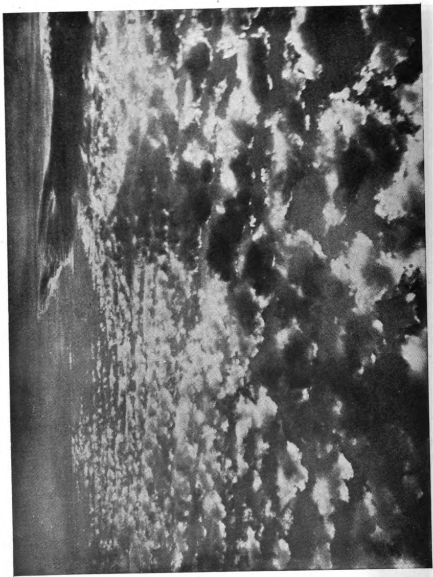
FIGURE 54. Alto-cumulus. (A. J. Weed, photo.)
