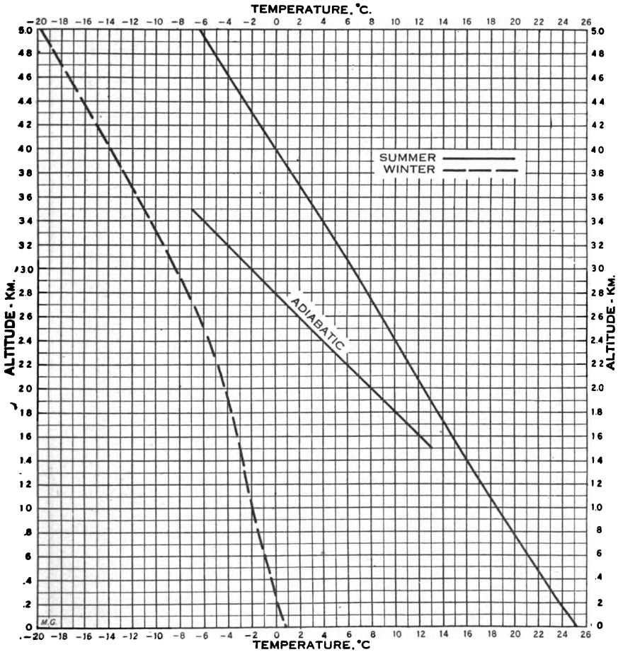
FIGURE 25. Mean summer and winter free air temperature gradients, °C, above Mount Weather, Va. (Extended to sea level.)
