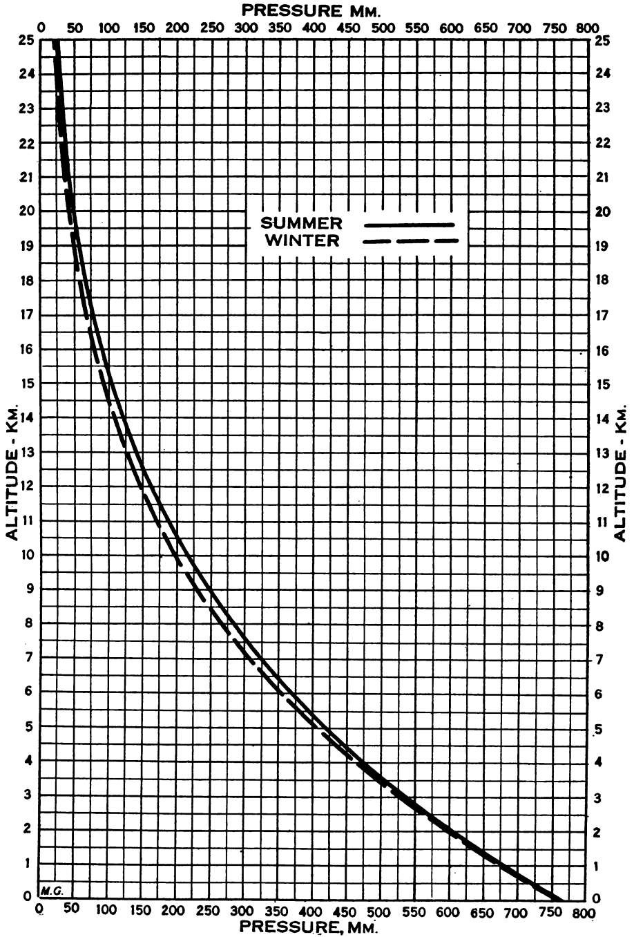
FIGURE 38. Mean summer and winter free air pressures, mm., from sounding balloon records in the Central and Western States.
