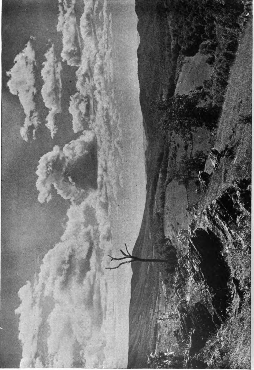
FIGURE 58. Fracto-cumulus, in Monroe Co., W. Va., Peters Mountain to left. (L. W. Humphreys, photo.)
