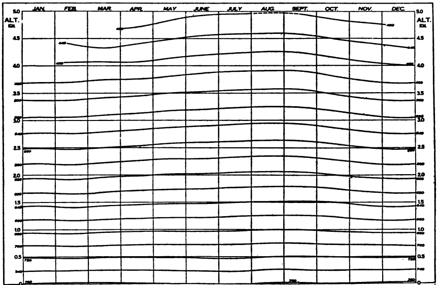
FIGURE 36. Mean annual march of free air pressures, mm., above Mount Weather, Va. (Extended to sea level.)
