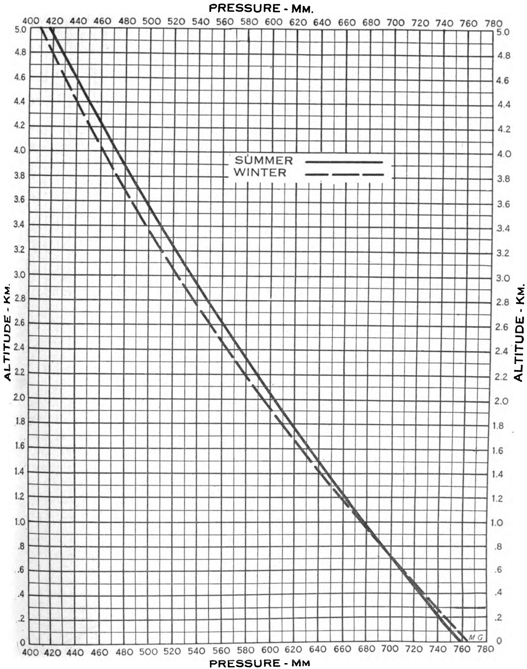
FIGURE 37. Mean summer and winter free air pressures, mm., above Mount Weather, Va. (Extended to sea level.)
