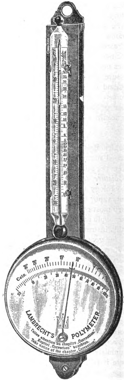
FIGURE 12. Lambrecht's Hygrometer.
