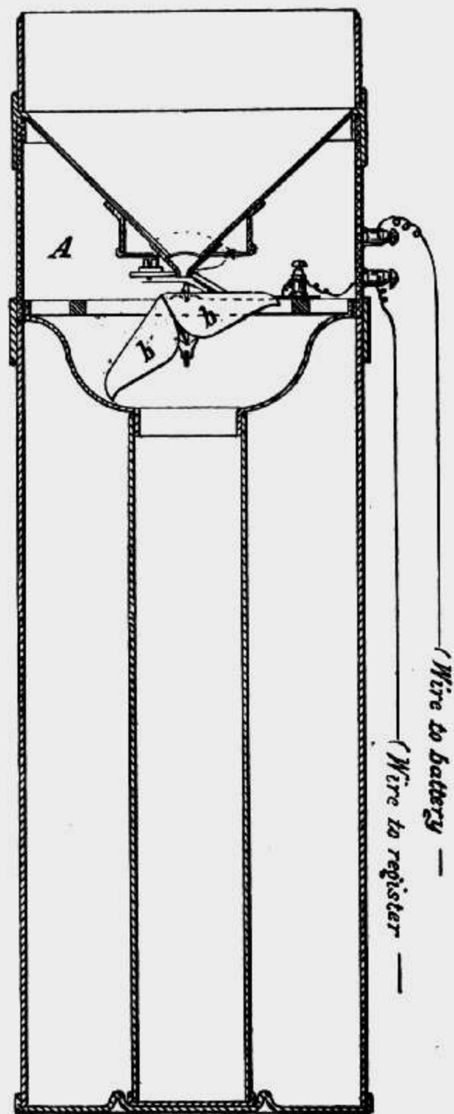
Vertical Section.
