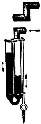
Lind's Portable Anemometer.
