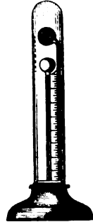
Leslie's Photometer.
