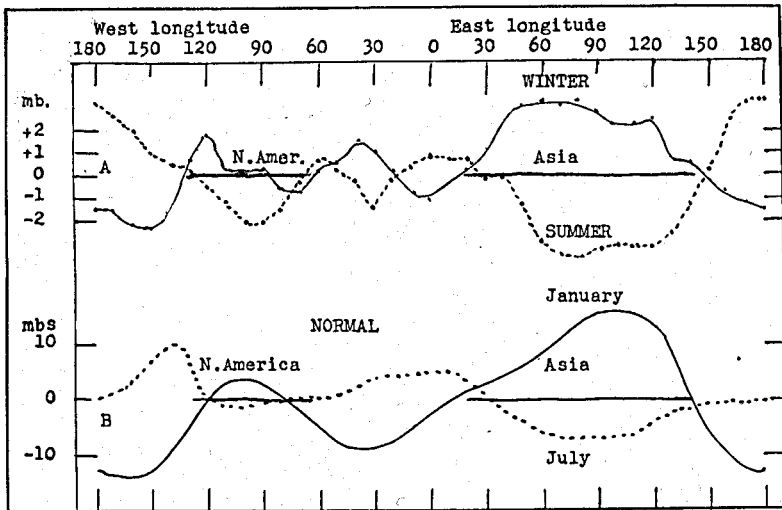
FIG. 11.—A, mean monthly changes in pressure at 50° N. latitude for the winter half-year and for the summer half-year accompanying sunspot changes of 10 or more in relative sunspot numbers; B, normal monthly pressure in January and July at 50° N. latitude in different longitudes.
