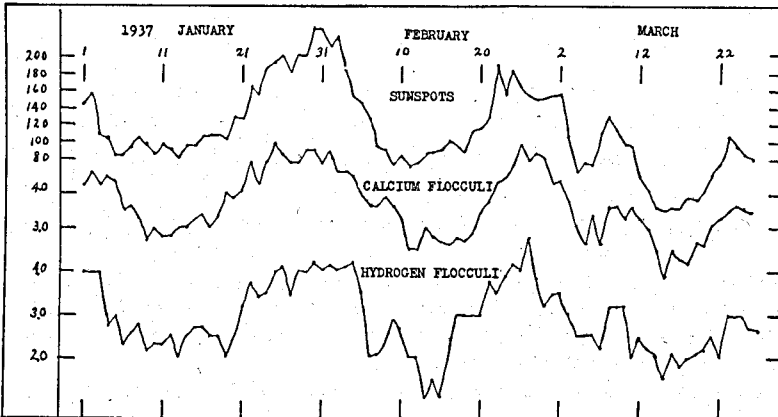
FIG. 10.—Comparison of day-to-day observations of sunspots, calcium flocculi, and hydrogen flocculi.
