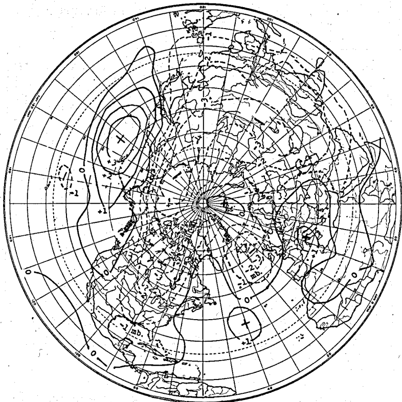
FIG. 12.—Monthly changes in pressure accompanying monthly increases in sunspots, summer half-year.
