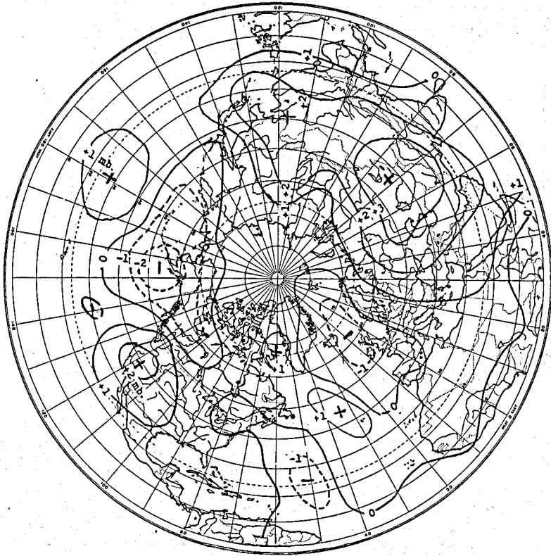
FIG. 13.—Monthly changes in pressure accompanying monthly increases in sunspots, winter half-year.
