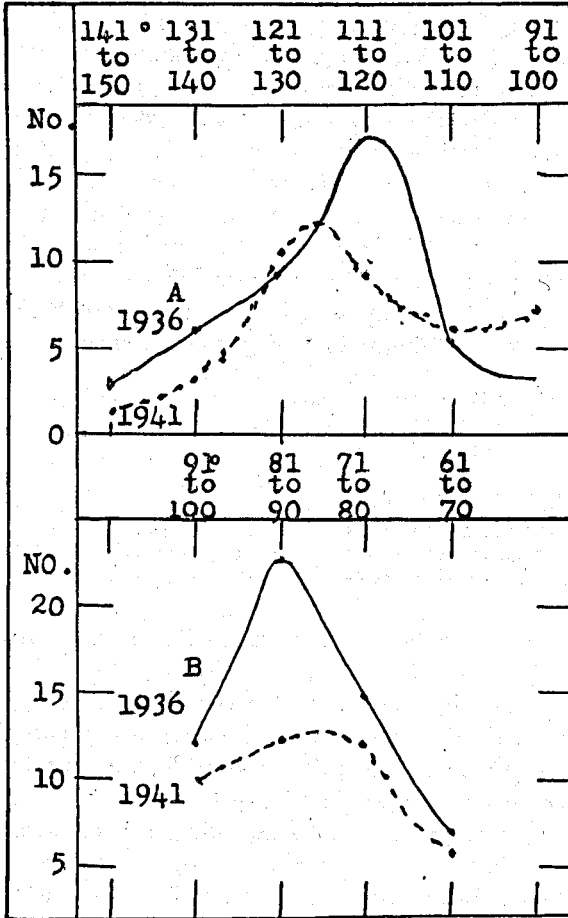
FIG. 8.—A, frequency of origin of anticyclones at different longitudes in North America north of 60° latitude, 1936 and 1941; B, frequency of origin of cyclones in the eastern United States and adjacent oceans south of 40° latitude, 1936 and 1941.
