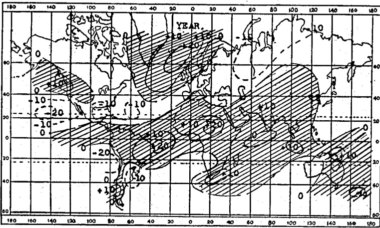
FIG. 16.—Distribution of differences of precipitation between sunspot maximum and sunspot minimum. Shaded areas show greater rainfall at sunspot maximum. Figures indicate percentages of normal.
