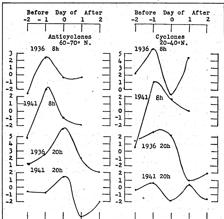
FIG. 7.—Mean daily changes in sunspots on days of origin of anticyclones and cyclones in North America and on the 2 days preceding and following. 8 h = by morning map; 20 h = by evening map.
