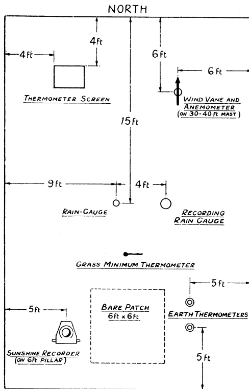
Recommended Layout of a Meteorological Station
