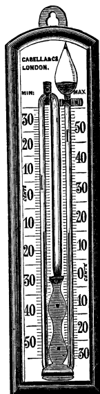
Six's Thermometer , opal glass or zinc scale, mounted on hardwood back, with magnet
