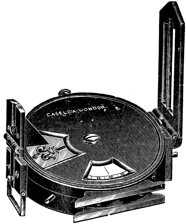
Clinometer Compass
