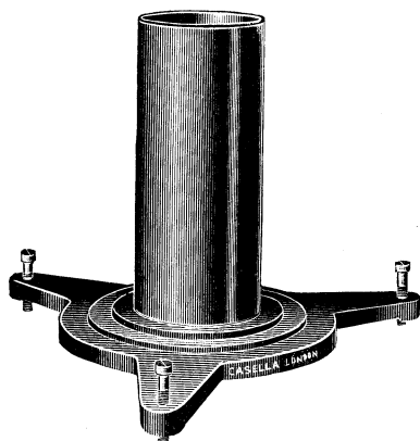
Still Well
