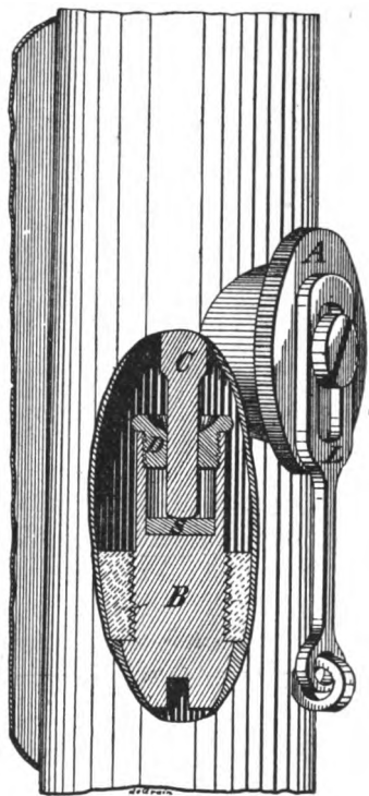
FIG. 5.—Anemometer bearings.
