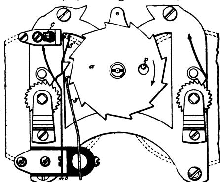
FIG. 14.—Five minute wind and sunshine clock contact.
