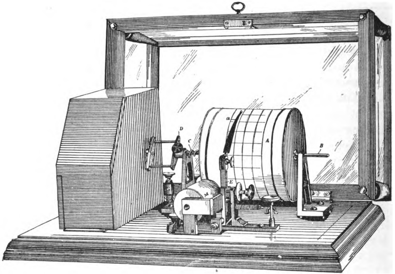
FIG. 10.—Single register.
