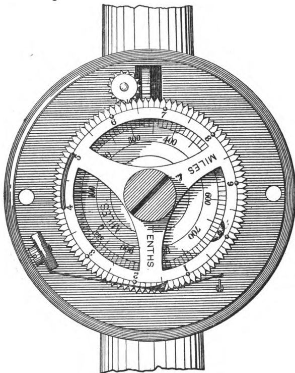
FIG. 4.—Anemometer dials.
