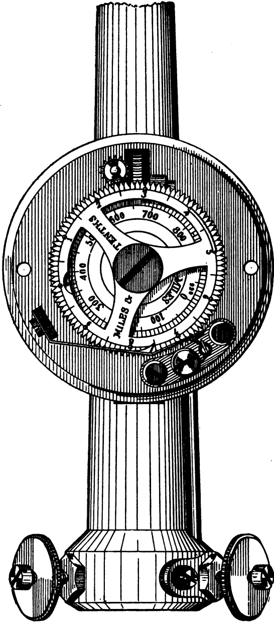
FIG. 8.—Improved anemometer.
