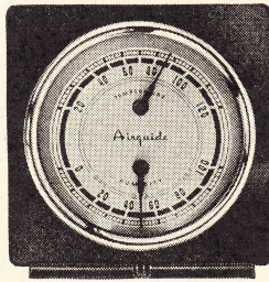
No. 103. THERMOMETER-HYGROMETER Tells both temperature and humidity May be used on desk or mounted on wall Brass finished bezel Height 3½", width 3¼", depth 1¼" Available in black, ivory or maroon plastic cases A neat and trim little instrument that will keep you posted on room temperature and humidity. The JUNIOR is inexpensive but finely made for accuracy of performance. Easel is designed to provide for desk use or wall mounting. A choice of three case colors (see listing below) permits selection which will best fit any room decorating color scheme. No. 103-A. Black case No. 103-B. Ivory case No. 103-C. Maroon case Price Each.....Retail $2.00 List $2.40
