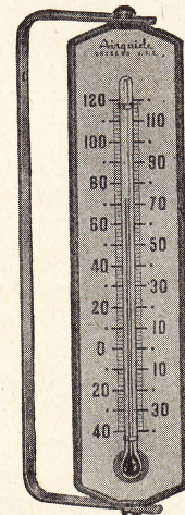
No. 402. OUTDOOR THERMOMETER Easily read numerals and calibrations Plated mounting bracket Adjustable to maximum visibility White vitreous enamel scale Magnifying tube with non-fading red fluid Height 7¾", width 1⅝" Maximum quality at popular price is represented in this attractive outdoor unit. The contrasting black figures and calibrations against the white enamel scale afford easy readability. No. 402. Price Each...Retail $2.00 List $2.40
