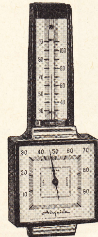
No. 101. THERMOMETER-HYGROMETER Shows temperature and relative humidity Designed for convenient wall mounting Black bakelite case, polished chrome trim Highly visible satin silver dial and scale Height 7¾", width 2¾", depth 1⅝" A smart and useful home or office appointment The sparkling design and easy readability of the ETON has made it one of the favorite models in the AIRGUIDE line. The glossy black plastic case set off by polished chrome trim fits it handsomely into any decorative scheme. No. 101. Price Each.....Retail $5.00 List $6.00
