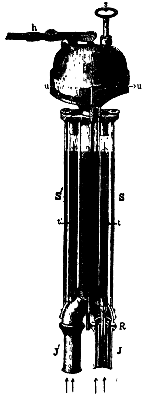
Fig. 2.—Assmann's Psychrometer.
