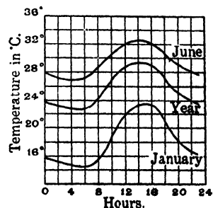
Fig. 27.—Diurnal variation of temperature at Alipore.
