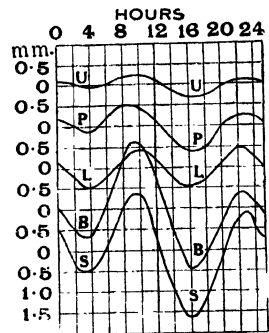
Fig. 29.— Diurnal variation of pressure at different latitudes.
