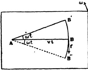
Fig. 38.—Illustration of the Corioli Force.
