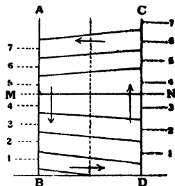
Fig. 37—Illustration of production of wind
