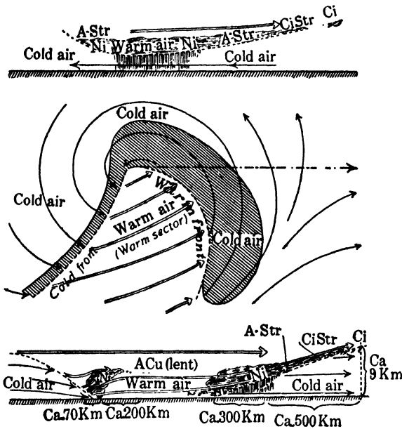
Fig. 46.—Structure of an idealised cyclone.
