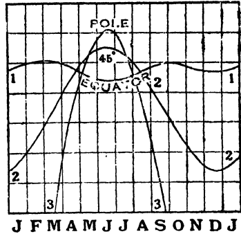
Fig 20.—Annual variation of insolation at different latitudes.
