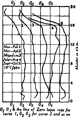
Fig. 22. - Variation of mean lapse-rate with height over Agra in different seasons.
