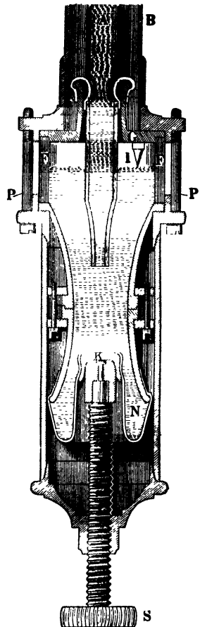
Fig.* 4(b).—Cistern of the barometer.
