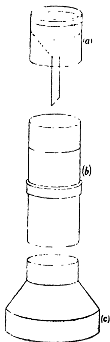
Fig. 13.—Symon's raingauge.
