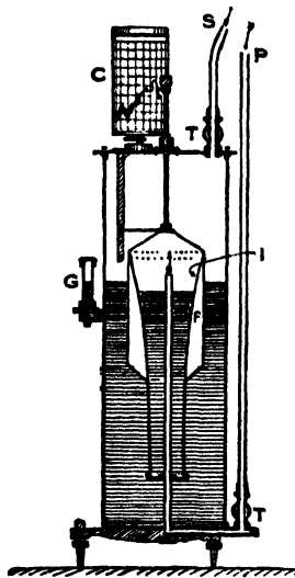
Fig. 8.—Dines' pressure-tube anemometer. (From 'Meteorology' by A.E.M. Geddes, Blackie & Son Limited).
