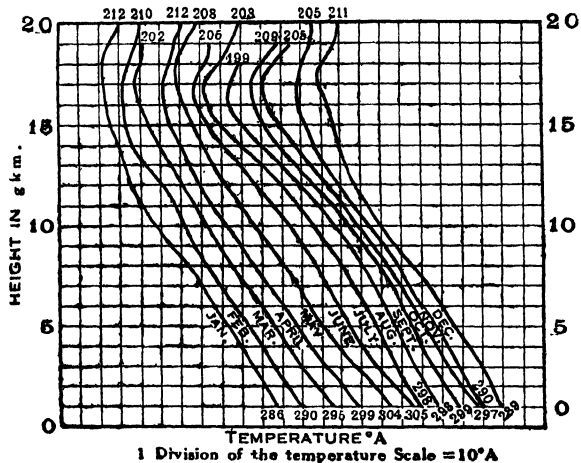
Fig. 21.—Vertical distribution of monthly mean temperatures over Agra.
