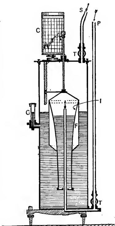
Fig. 36.—Section Diagram of Recording Apparatus of Dines' Pressure-tube Anemometer
