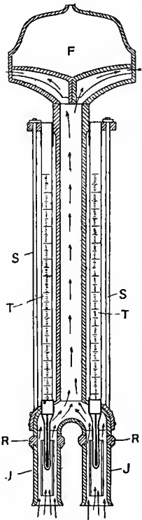
Fig. 13.—Assmann's Ventilation Thermometer
