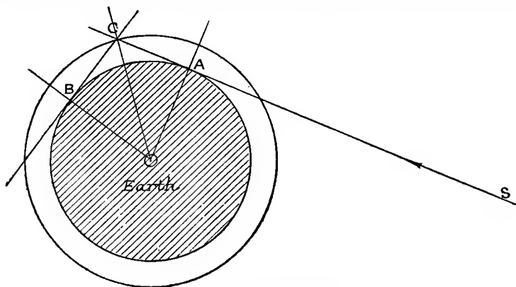
Fig. 5.—Cause of Twilight
