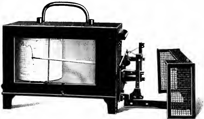
Fig. 53.—Hair Hygrometer, M.O. pattern, with guard removed to show bundle of hairs and lever
